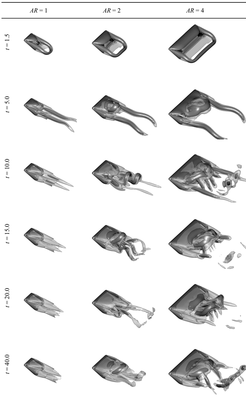
FIGURE 4. Top-port views of the wake vortices behind rectangular plates of AR = 1, 2 and 4 at \alpha = 30^\circ and Re = 300 . Shown are the iso-surface of \|\omega\|_2 = 3 in light grey with vortex cores highlighted by the iso-surface of Q = 3 in dark grey.
