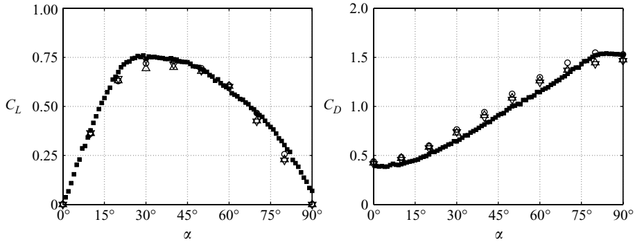
FIGURE 3. Lift and drag coefficients for a rectangular plate of AR=2 at Re=100 . Data from the oil tow tank experiments are shown with \blacksquare and results from numerical simulations are presented with (\circ) , (\Delta) and (\nabla) for grid sizes of 125 \times 55 \times 80 , 150 \times 66 \times 96 and 200 \times 88 \times 128 , respectively.
