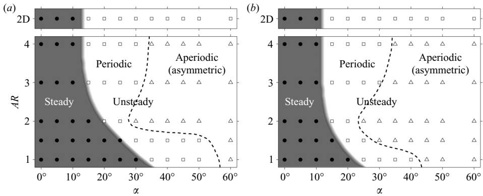
FIGURE 10. Stability of the wake for a range of \alpha and AR at (a) Re = 300 and (b) Re = 500 . Symbols (●), (□) and (△) denote steady, unsteady periodic and unsteady aperiodic wakes at large time. The shaded area and the dashed line approximately represent the region of stability and the transition from periodic to aperiodic shedding, respectively. Shown at the top are the two-dimensional findings.
