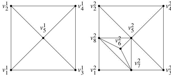
Fig. 1. The two regular complexes \Delta_1 (on the left) and \Delta_2 (on the right) of the square [0, 1]^2 . Every function x, y and x \oplus y is linear over each simplex of \Delta_1 and \Delta_2 .
