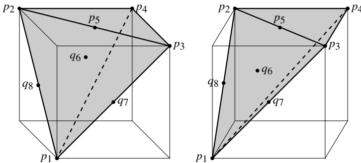
Fig. 2. The convex polytope \mathcal{D}_\Phi (in two perspectives) for \Phi = \{x, y, x \oplus y\} , and its extremal points p_1, p_2, p_3 and p_4 .
