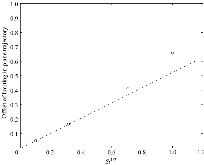
FIGURE 12. The in-plane critical offset ((z_{sep}^{-\infty})^c St^{1/2}) values obtained from numerical integration of the trajectory equation, (4.2) with \theta = \pi/2 , are plotted as a function of St^{1/2} ; the dashed line represents the theoretical approximation (4.40).
