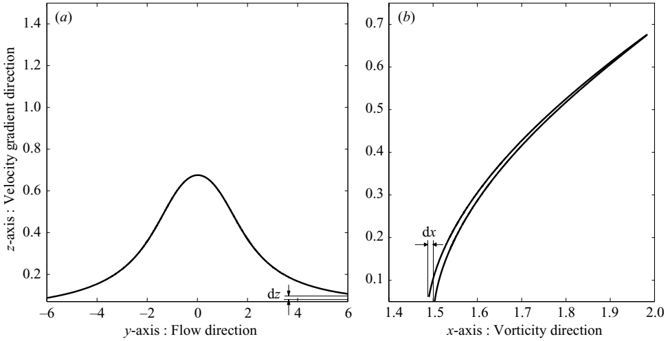
FIGURE 20. Limiting off-plane open trajectory for St = 0.1 with x^{-\infty} = 1.5 and z^{-\infty} = 0 : (a) yz - and (b) xz -projections.
