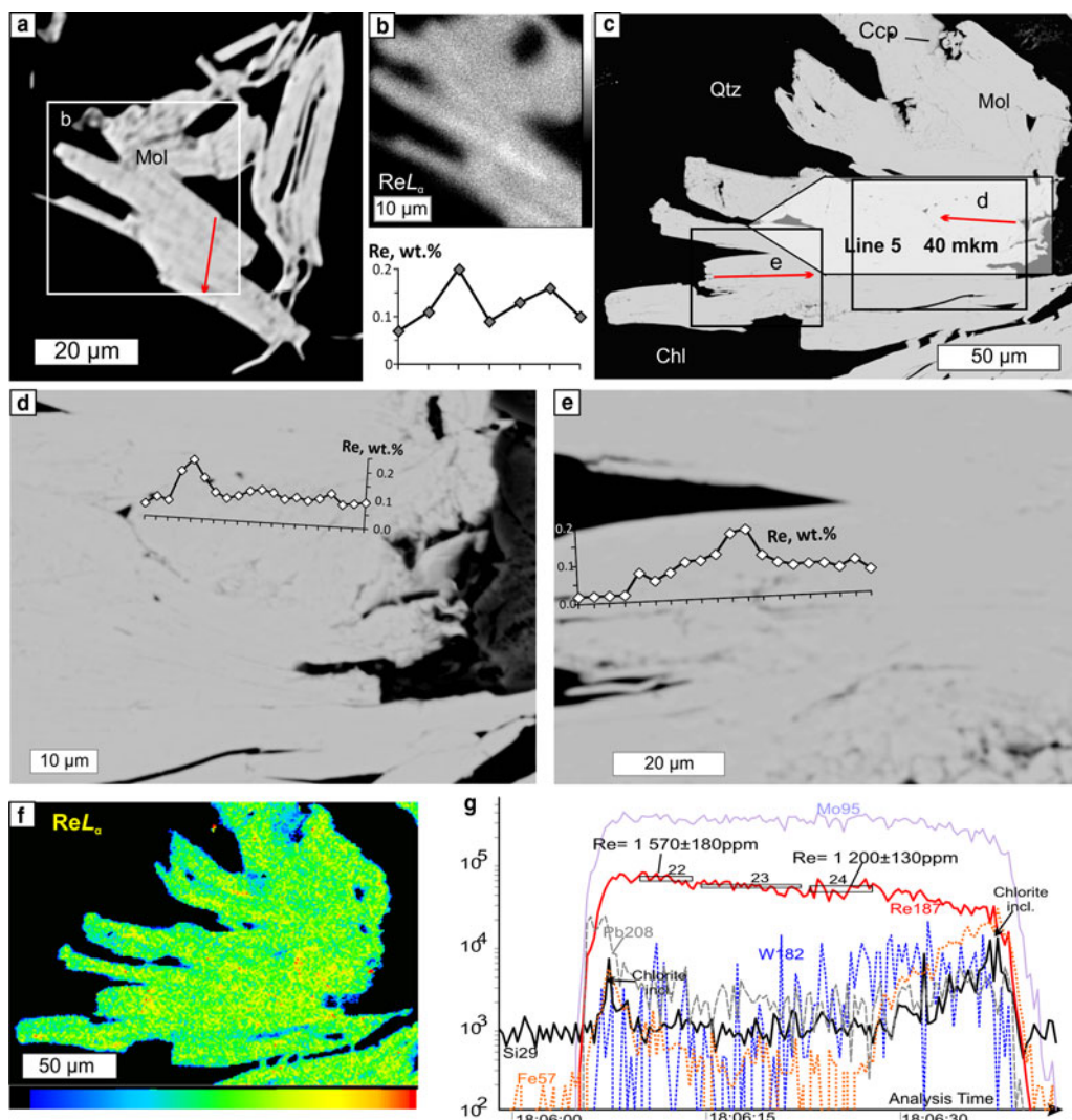
FIG. 5. Molybdenite from Birgilda, samples Bir-42/84 (a,b) and Bir-4905/294.4 (c). (a) SEM image of molybdenite flakes; (b) \text{ReL}\alpha X-ray map of a fragment of a and the EMPA profile across the flake (the position is indicated by a red arrow); (c) SEM image of a molybdenite 'semi-rosette' with the positions of the EMPA and LA-ICP-MS profiles; (d,e) fragments of (c) with the EMPA profiles; (f) \text{ReL}\alpha X-ray map of (c); (g) LA-ICP-MS spectra for line 5.
