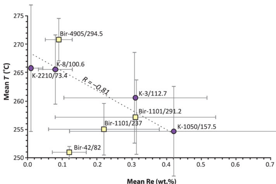
FIG. 12. Mean T ( ^{\circ}\text{C} ) vs. mean wt.% Re from the EPMA analyses (Table 3). Error bars are shown for 1 sd. The temperature was calculated after Kotelnikov et al. (2012) (Table 2). The correlation coefficient is given for the whole dataset excluding sample Bir-42/82.
