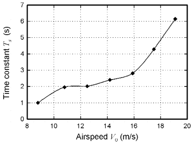
Figure 21. Spiral mode characteristic.
