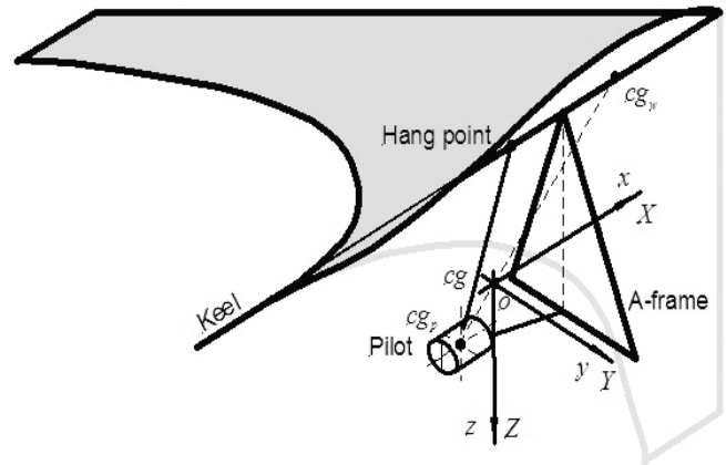
Figure 1. Hang glider body axis system.
