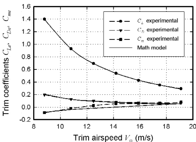
Figure 15. Trim lift, drag and pitching moment coefficients comparison.
