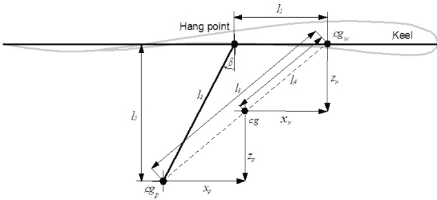
Figure 6. Longitudinal control geometry.
