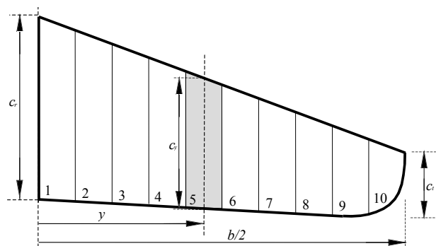
Figure 8. Wing panel segment model.
