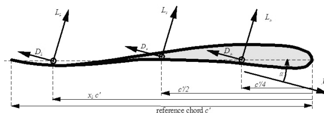
Figure 9. Aerofoil lift and drag distribution.
