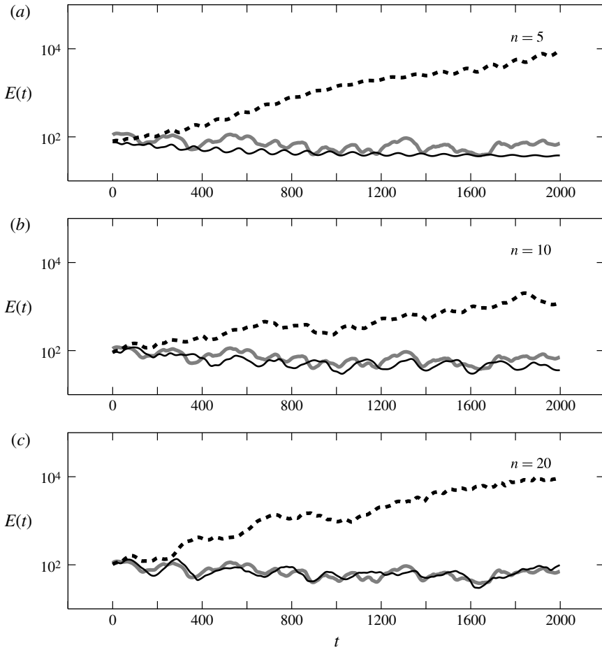
FIGURE 11. The evolution of the instantaneous turbulent kinetic energy of the mixing layer as predicted by standard POD-based Galerkin ROMs (dashed black lines) and the new Galerkin ROMs (solid black lines); DNS (thick grey lines).
