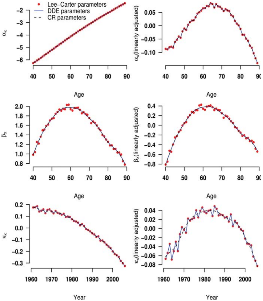
Figure 3. Parameter plots for \alpha_x , \beta_x and \kappa_x (left column), and the same parameters after linear adjustment (right column); the original Lee-Carter parameters are shown as solid dots, while the DDE parameters are shown by a solid line and the CR parameters are shown by a dashed line; the linear-adjusted plots show the same coefficients on the left after subtracting a fitted straight line; they show, for example, that the pattern of \alpha_x by age is not as linear as it seems (ONS data)
