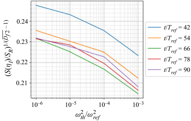
Figure 18. Plot of (S(\eta_T)/S_R)^{1/(\overline{D}_{f2}-1)} as a function of \omega_{th}^2/\omega_{ref}^2 at different times t/T_{ref} .
