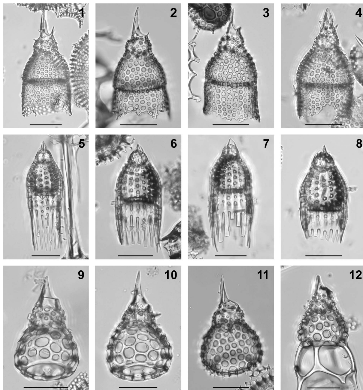
Figure 7. Composite light micrographs of radiolarian species from ODP Site 1260 (Demerara Rise, western equatorial Atlantic). (1–4) Albatrossidium annikasanfilippae n. sp.: (1) holotype, ODP 1260A-12R-3W, 55–57 cm, USTL 3512-1, Y39/1; (2) ODP 1260A-13R-4W, 55–57 cm, USTL 2854-5, X67/4; (3) ODP 1260A-13R-4W, 55–57 cm, USTL 2854-2, O66/1; (4) ODP 1260A-9R-3W, 55–57 cm, USTL 3477-2, L56/3. (5–8) Phormocyrtis lazari n. sp.: (5) holotype, ODP 1260A-9R-2W, 55–57 cm, USTL 3474-1, T40/4; (6) ODP 1260A-9R-3W, 55–57 cm, USTL 3480-1, M35/1; (7) ODP 1260A-9R-4W, 55–57 cm, USTL 3482-2, W36/3; (8) ODP 1260A-9R-4W, 55–57 cm, USTL 3481-3, E38/3. (9–12) Podocyrtis (Lampterium) puellasinensis Ehrenberg, 1874: (9) ODP 1260A-6R-2W, 55–57 cm, USTL 3420-1, U56/1; (10) ODP 1260A-9R-4W, 55–57 cm, USTL 3484-3, D47/3; (11) ODP 1260A-12R-1W, 55–57 cm, USTL 2851-4, C47/4 (mirrored). (12) Podocyrtis (Lampterium) goetheana (Haeckel, 1887), focus on the cephalothorax, ODP 1260A-8R-2W, 54–56 cm, USTL 3461-2, S49/1 (mirrored). All scale bars equal 50 \mu m.
