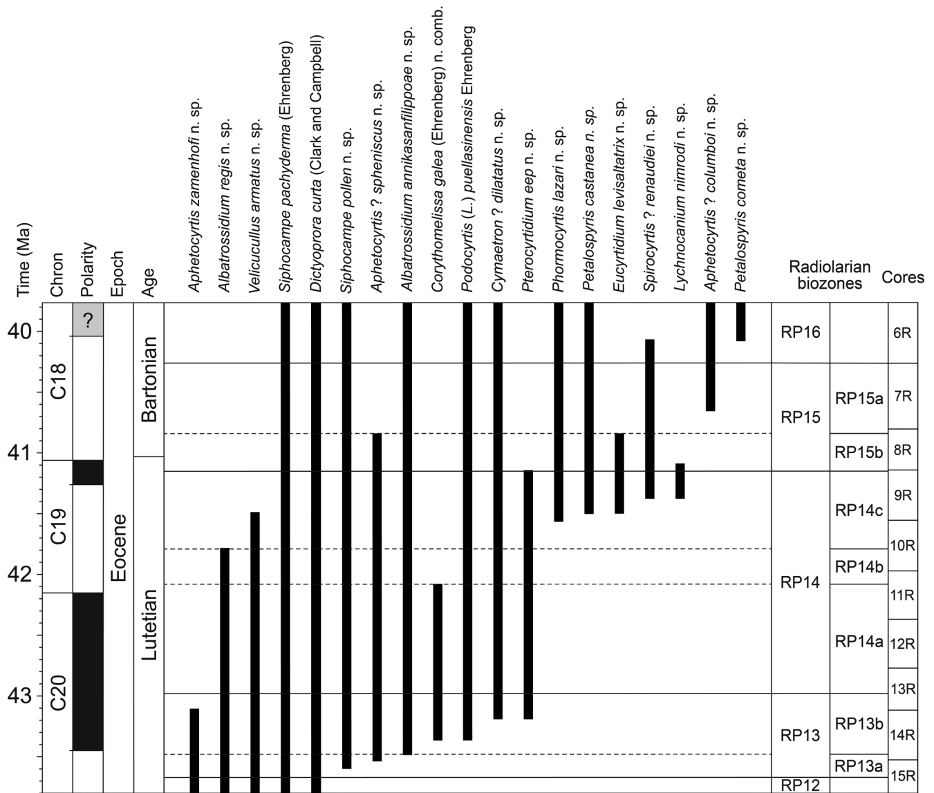
Figure 2. Range chart of 19 selected radiolarian species from the middle Eocene of ODP Site 1260 (Demerara Rise, western equatorial Atlantic). Geomagnetic timescale after calibration of Saganuma and Ogg (2006); radiolarian biozonations after Meunier and Danelian (2022).
