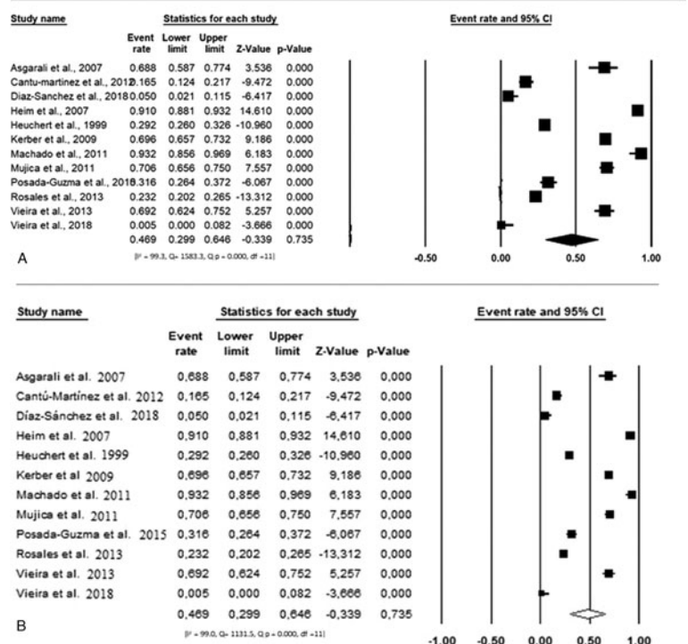
Fig. 4. Forest plot of the prevalence estimates due to equine piroplasms in the Americas. Prevalence due to T. equi in the Americas is illustrated in (A) while estimates due to B. caballi are shown in (B). Note: The squares show the individual point estimate. The diamond at the base indicates the pooled estimates from the total studies.
