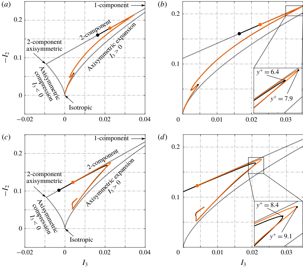
FIGURE 19. Reynolds stress anisotropy-invariant map for the adiabatic duct (—) and the heated duct (—, orange) evaluated at (a,b) 2z/L_z = 0 and (c,d) 2z/L_z = 0.95 along the y -line from the heated wall to the duct centre, and limiting states defined by the Lumley triangle. The wall location is represented by \bullet and \bullet (orange) respectively.
