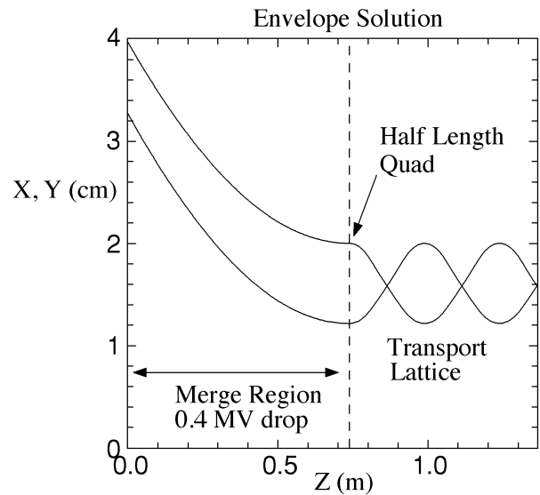
Fig. 6. Simulation of the beam envelope in the merging section of the multiple aperture injector and the first few quadrupoles of the accelerator.
