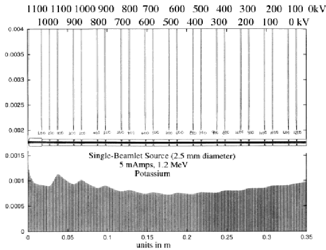
Fig. 5. EGUN simulation of a single beamlet through an Einzel lens transport lattice.
