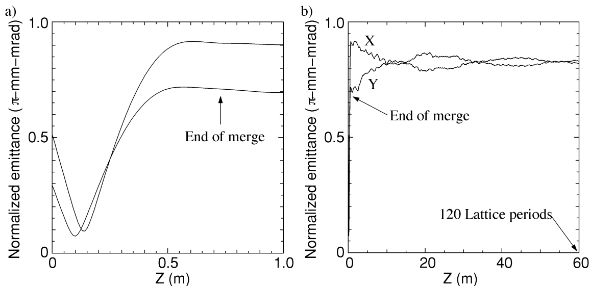
Fig. 7. Plot of x and y normalized emittances as a function path length through the merging section and the beginning of the accelerator.
