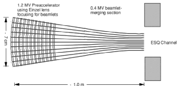
Fig. 4. Schematic diagram of multiple aperture source injector to produce one 500-mA beam.
