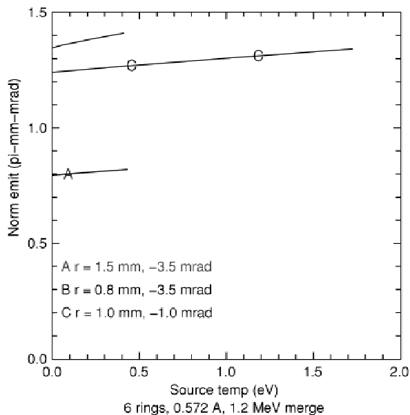
Fig. 8. Plot of normalized emittance as a function of ion temperature of the source.
