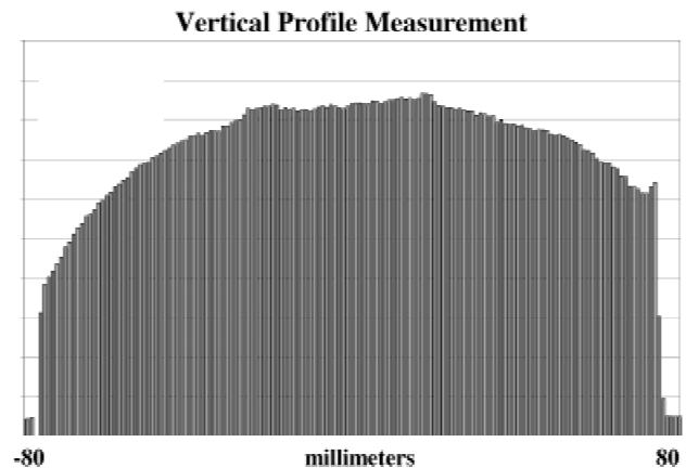
Fig. 2. Vertical profile measurement of HCX beam at end of ESQ injector after modifications to source geometry. The y-axis units are arbitrary.
