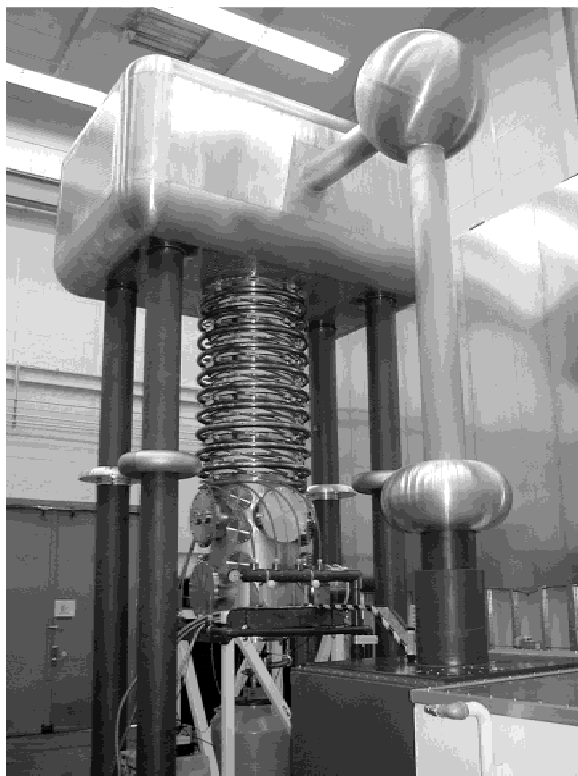
Fig. 3. Picture of STS-500, a newly commissioned 500-kV ion source test stand.
