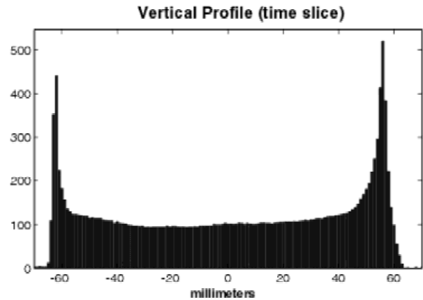
Fig. 1. Vertical profile measurement of ILSE beam at end of ESQ injector. The profile is for one time slice during the middle of the beam. The y-axis units are arbitrary.
