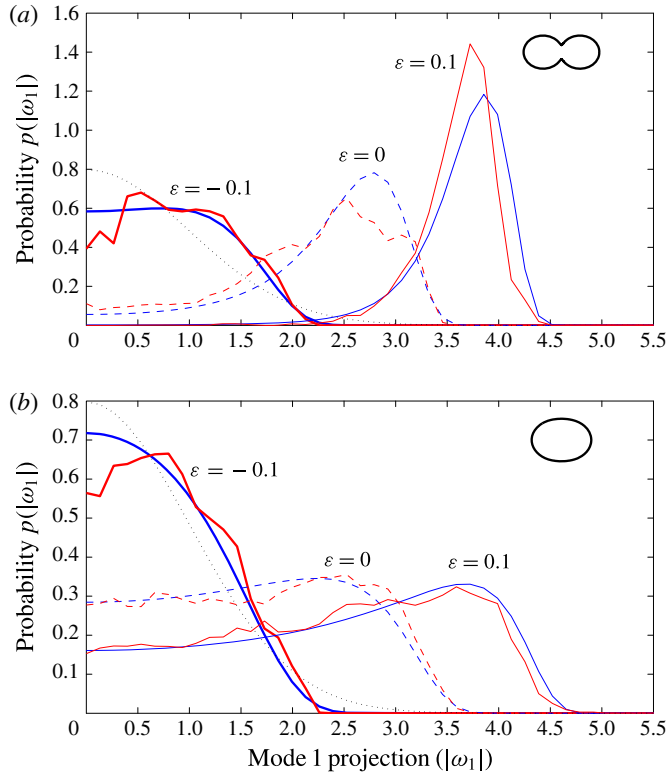
FIGURE 5. (Colour online) Comparison between theoretical predictions ((3.15), blue curves) of p_\varepsilon(|\omega_1|) and DNS ((2.2), red curves): (a) domain A; (b) domain B. Three different energy levels ( \varepsilon = -0.1, 0, 0.1 ) are shown (2.2).
