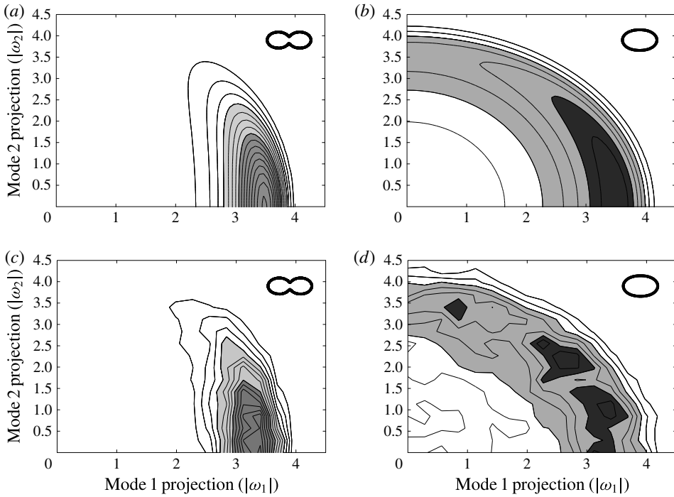
FIGURE 6. Contour plots comparing p_\epsilon(|\omega_1|, |\omega_2|) (a,b) predicted by the theory (3.16) with (c,d) statistics compiled from the DNS (2.2): (a,c) domain A; (b,d) domain B. The energy is fixed at \epsilon = 0.05 .
