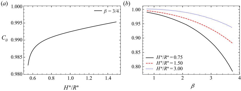
Figure 2. Evolution of the ratio C_\theta \equiv \zeta_B/\theta_j(\zeta_B) for ( N = 1, R^* = 7 ): (a) C_\theta as a function H^*/R^* for \beta = 3/4 , and (b) as a function of \beta for different H^*/R^* .
