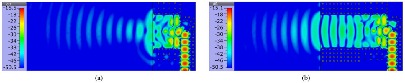
Fig. 2. Simulated electric field distribution of the designed antenna structures with SIW feed and radiation into free-space for (a) antenna 1 and (b) antenna 2.
