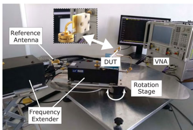
Fig. 6. Measurement setup for the characterization of the radiation pattern and antenna gain.
