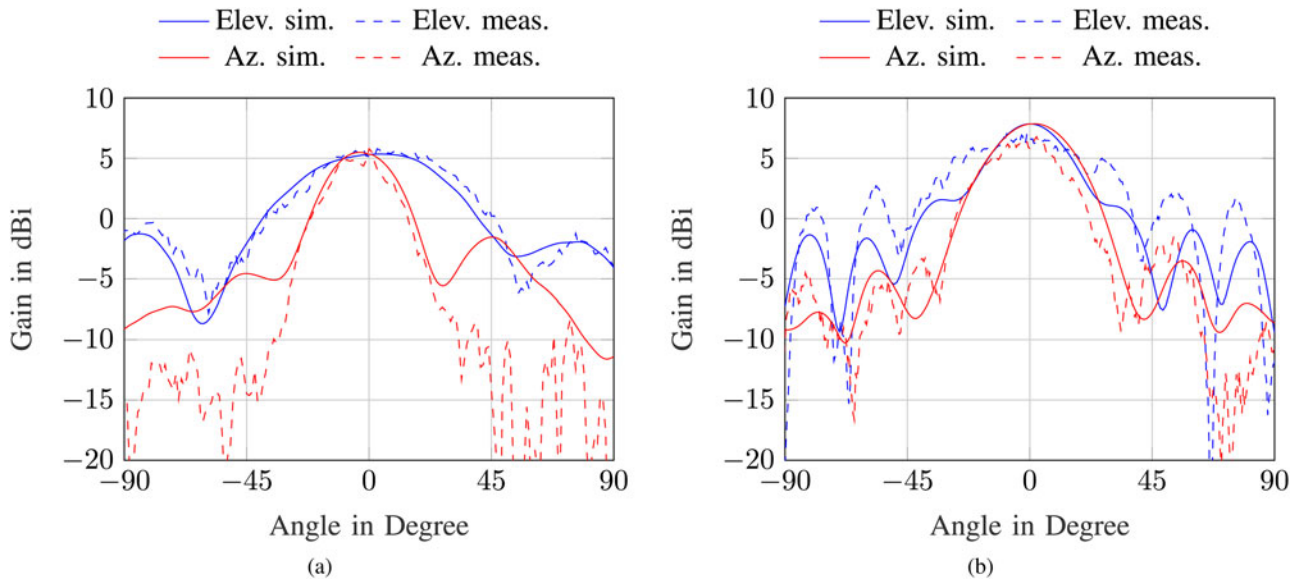
Fig. 3. Simulated and measured radiation patterns in azimuth and elevation for (a) antenna 1 and (b) antenna 2 at 122.5 GHz.
