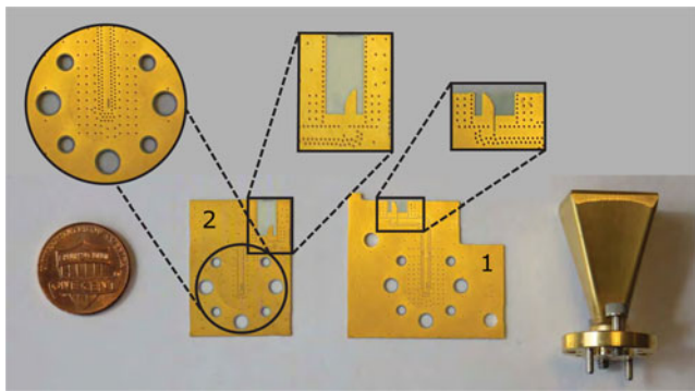
Fig. 5. Photograph of the fabricated antennas 1 and 2 with highlighted transition from SIW to rectangular waveguide and the antenna structures together with a 24 dBi horn antenna in D band.
