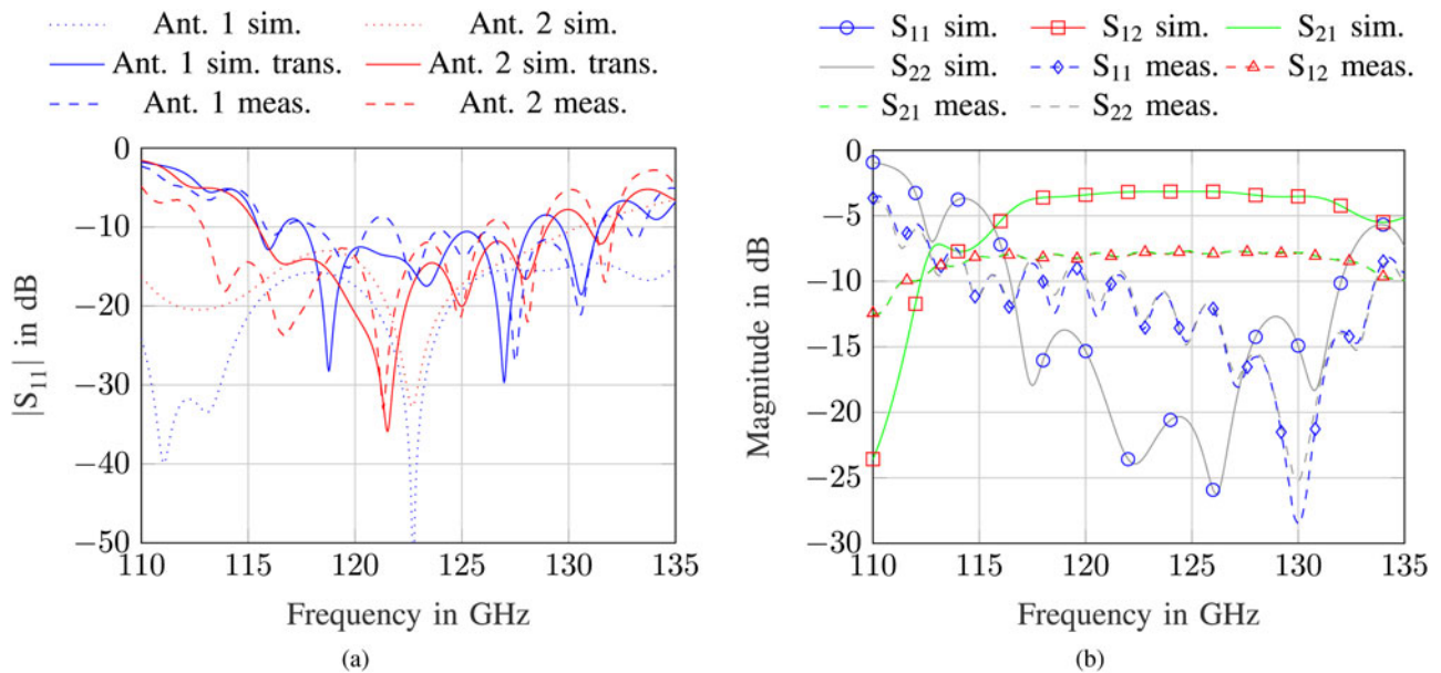
Fig. 4. (a) Simulated and measured free-space reflection coefficient for both antenna designs and (b) simulated and measured S-parameters for the transition in back-to-back configuration.
