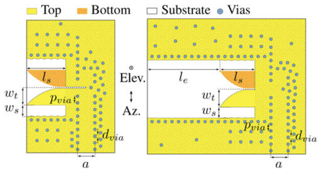
Fig. 1. Layout of the SIW fed vivaldi-shaped antenna 1 (left) and extended substrate antenna 2 (right) with the main design parameters (top view).
