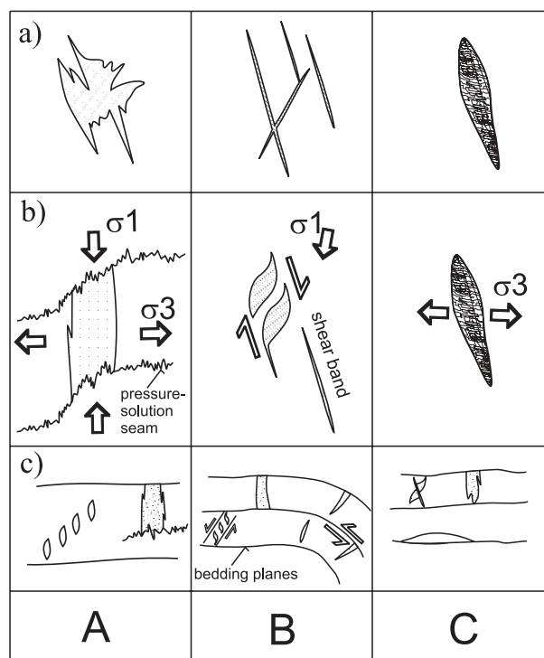
Figure 4. Example schemes of main structural features of the classified calcite veins (A, B, C): (a) the most common shape of veins; (b) typical vein geometry with respect to the stress fields; (c) position and orientation of veins in sedimentary beds.
