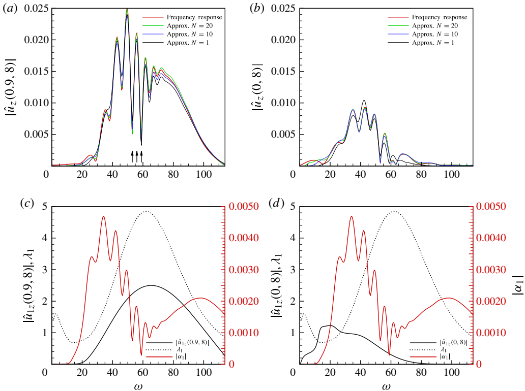
FIGURE 14. (a,b) Comparison of true frequency response based on (4.3) with approximations based on N = 1, N = 10 and N = 20 singular modes (see (6.3)). Axial velocity component at (a) ( r = 0.9, z = 8 ) and (b) ( r = 0, z = 8 ). (c,d) Analysis of leading order response \hat{\mathbf{u}} = \alpha_1 \lambda_1 \hat{\mathbf{u}}_1 at (c) ( r = 0.9, z = 8 ) and (d) ( r = 0, z = 8 ). Here Re = 1600 and discretization D_1 .
