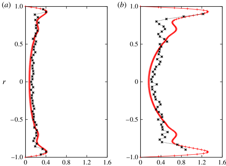
FIGURE 17. Comparison of radial profiles of optimal response |\hat{u}_1| obtained at \omega = 63.25 (for Re = 1600 ) with RMS of velocity fluctuations (obtained for Re = 1660 ). Two sections are investigated: (a) z = 7.93 , where the overall amplitude of the response has been chosen to match the experimental profile; and (b) z = 9.57 , where the profile of the response has been deduced from the structure of the leading optimal response. Discretization D_1 for stability computation. Experimental results reproduced from Cerqueira et al. (2009).
