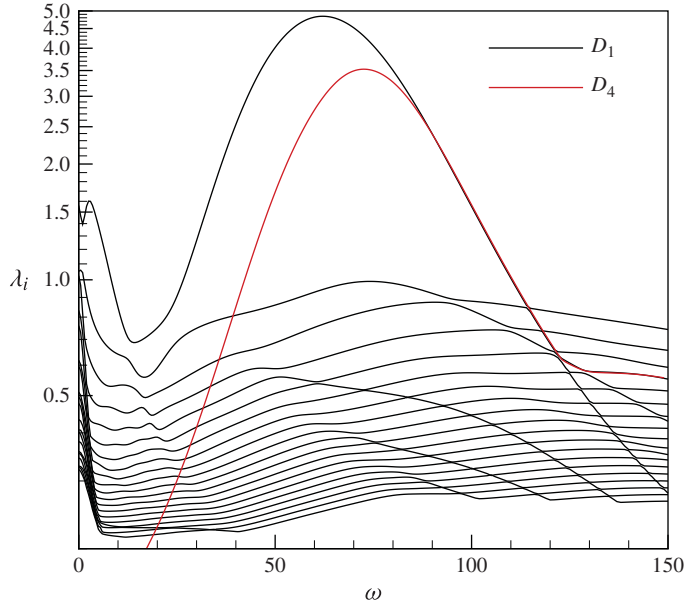
FIGURE 9. The 20 leading singular values \lambda_i for discretization D_1 (black solid lines) and leading singular value \lambda_1 for discretization D_4 (red solid line) as a function of frequency \omega . Re = 1600 .
