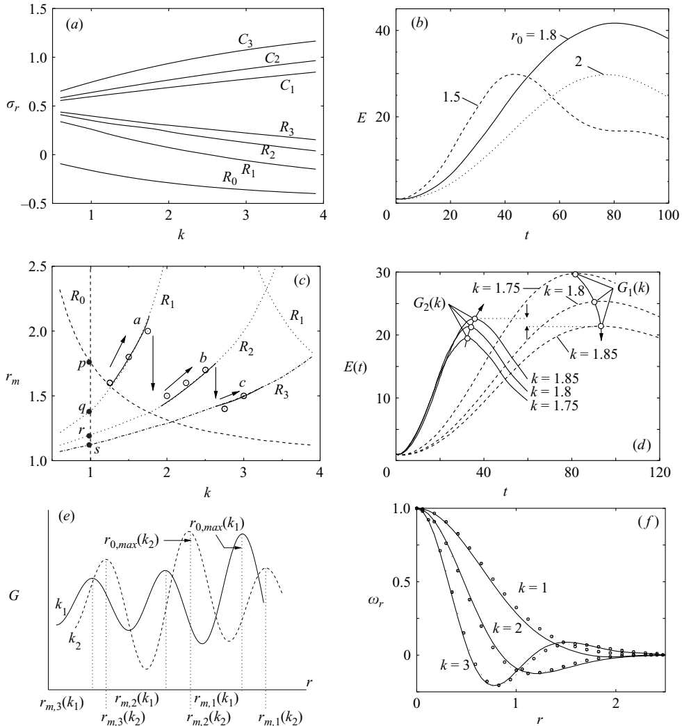
FIGURE 21. Top-hat vortex behaviour (a–e). (a) Dispersion curves. (b) E(t) evolution as function of ribbon radius r_0 , for k = 1.5 and Re = 10^4 . (c) The resonant radii r_m , where the mean-flow angular velocity V/r matches eigenmode frequency \sigma_r , for various eigenmode branches (broken lines R_0 – R_3 ); circles show the computed ribbon radial locations r_{0,max} . Arrows show discrete r_{0,max} jumps across different R_i branches, with solid lines showing the trends of r_{0,max} . Core \omega_z distributions at modes labelled i, ii, iii are plotted in figure 22. Once again, in this (r, k) -plane, broken lines show r_m(k) and symbols and solid lines denote r_{0,max}(k) . (d) E(t) evolution when ribbon radius r_0 equals r_m on R_1 (dashed lines) and on R_2 (solid) branches, for various k . The maximum values of E(t) , i.e. G , on R_1 and R_2 branches are indicated by curves with open circles G_1(k) and G_2(k) , respectively. (e) Sketch of the variations of G with ribbon radius r_0 at two k values k_1 and k_2 . At any k , local maxima of G occur at resonant radii r_m , and the global maximum of G corresponds to r_{0,max} . (f) Oseen-vortex optimal mode \omega_r profiles at time of peak amplification (lines), and Oseen-vortex eigenmode \omega_r (symbols), at three k values.
