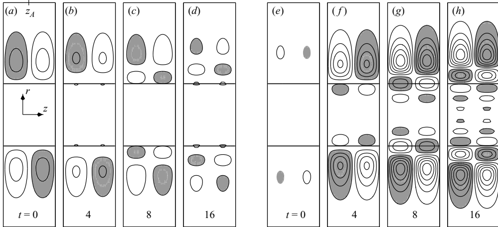
FIGURE 12. \omega_r (a–d) and \omega_\theta (e–h) contours for an Oseen vortex m=0 optimal mode, figure 11(b–d), at times t=0, 4, 8, 16 . In all cases, Re=2000, k=\pi ; contours are plotted with \omega_{min}=0.05 and \delta\omega=0.1 . Thick lines denote \Omega_z=0.5 (corresponding to r \approx 1.3 in figure 8a).
