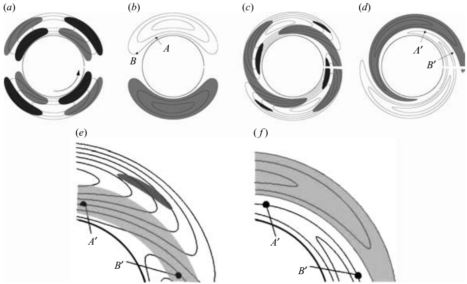
FIGURE 2. Contours of \psi (a,c) and \omega (b,d) at t=0 (a,b) and t=100 (c,d) illustrating the two-dimensional mechanism of transient growth cessation. Light-shaded regions in (a,c) denote uv < 0 and dark-shaded regions uv > 0 . Shaded regions in (b,d) denote negative \omega . Two fluid particles initially at A, B are advected to A', B', respectively, at t=100 . Close-up views of \psi contours (e) and \omega contours (f) at t=100 .
