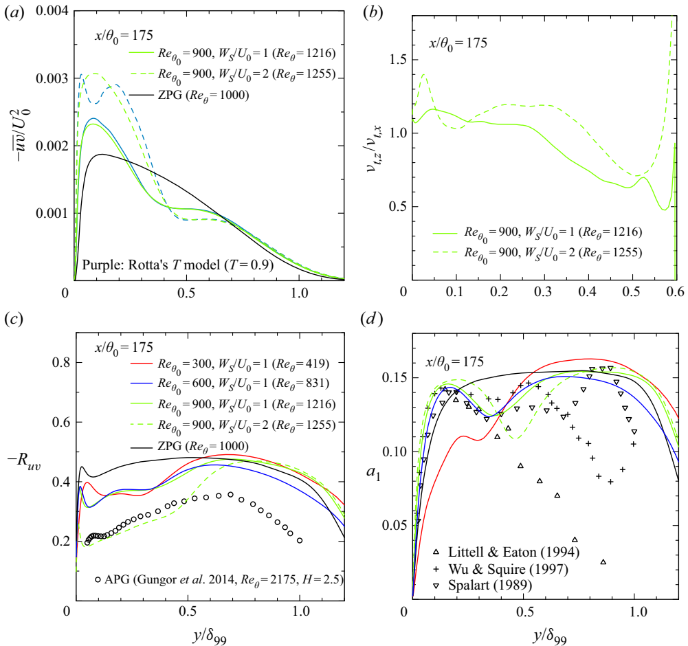
FIGURE 22. Distributions of the outer-normalized -\overline{uv} , the correlation coefficient -R_{uv} , the turbulent eddy viscosity ratio \nu_{t,z}/\nu_{t,x} and the structure parameter a_1 in the 3DTBL region ( x/\theta_0 = 175 ): (a) -\overline{uv}/U_0^2 for Re_{\theta_0} = 900 with W_S/U_0 = 1 and 2; (b) \nu_{t,z}/\nu_{t,x} for Re_{\theta_0} = 900 with W_S/U_0 = 1 and 2; (c) -R_{uv} for Re_{\theta_0} = 300, 600 and 900 with W_S/U_0 = 1 and Re_{\theta_0} = 900 with W_S/U_0 = 2 ; and (d) a_1 for Re_{\theta_0} = 300, 600 and 900 with W_S/U_0 = 1 and Re_{\theta_0} = 900 with W_S/U_0 = 2 . The data shown have been obtained with L_x, W_S = 100\theta_0 . Also plotted for comparison are the DNS data of a ZPG 2DTBL for Re_\theta = 1000 obtained in the present work.
