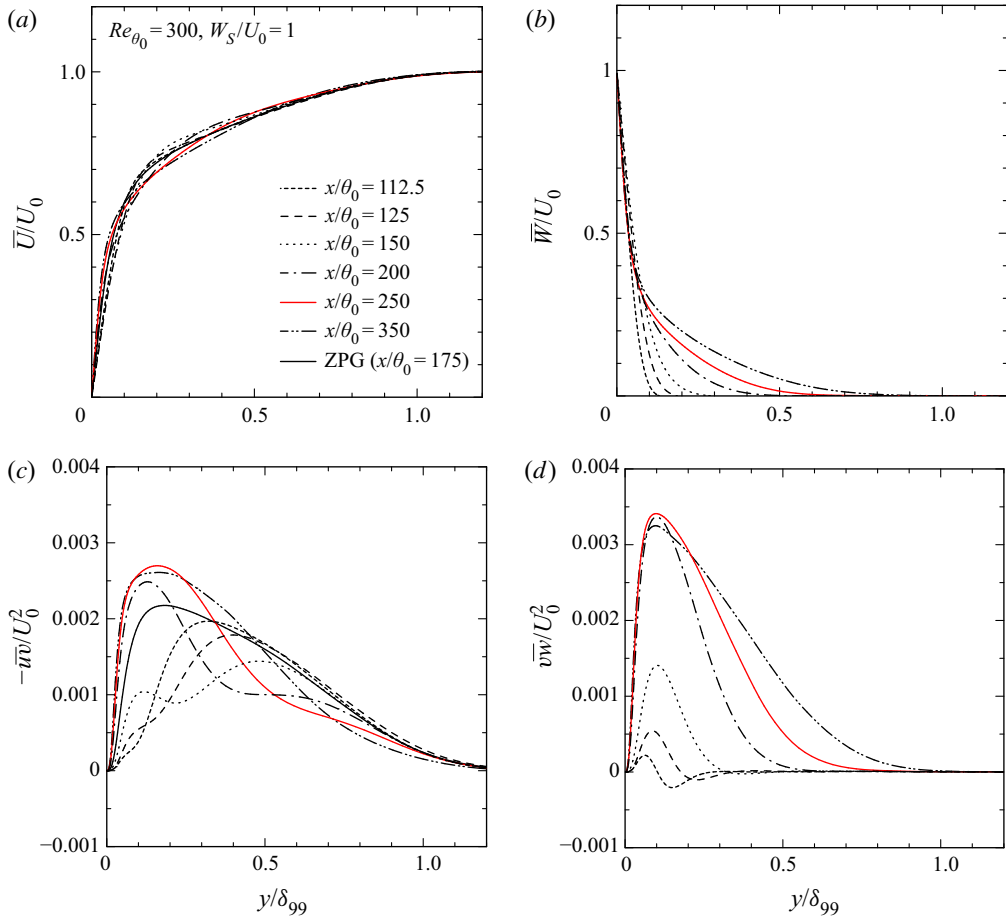
FIGURE 6. Distributions of normalized \bar{U} , \bar{W} , \bar{uv} and \bar{vw} in the 3DTBL region for Re_{\theta_0} = 300 with W_S/U_0 = 1 : (a) \bar{U}/U_0 ; (b) \bar{W}/U_0 ; (c) -\bar{uv}/U_0^2 ; and (d) \bar{vw}/U_0^2 . The red lines refer to the data at x/\theta_0 = 250 where a near-plateau has been established in C_{f,x} . The data shown have been obtained with L_{x,W_S} = 300\theta_0 .
