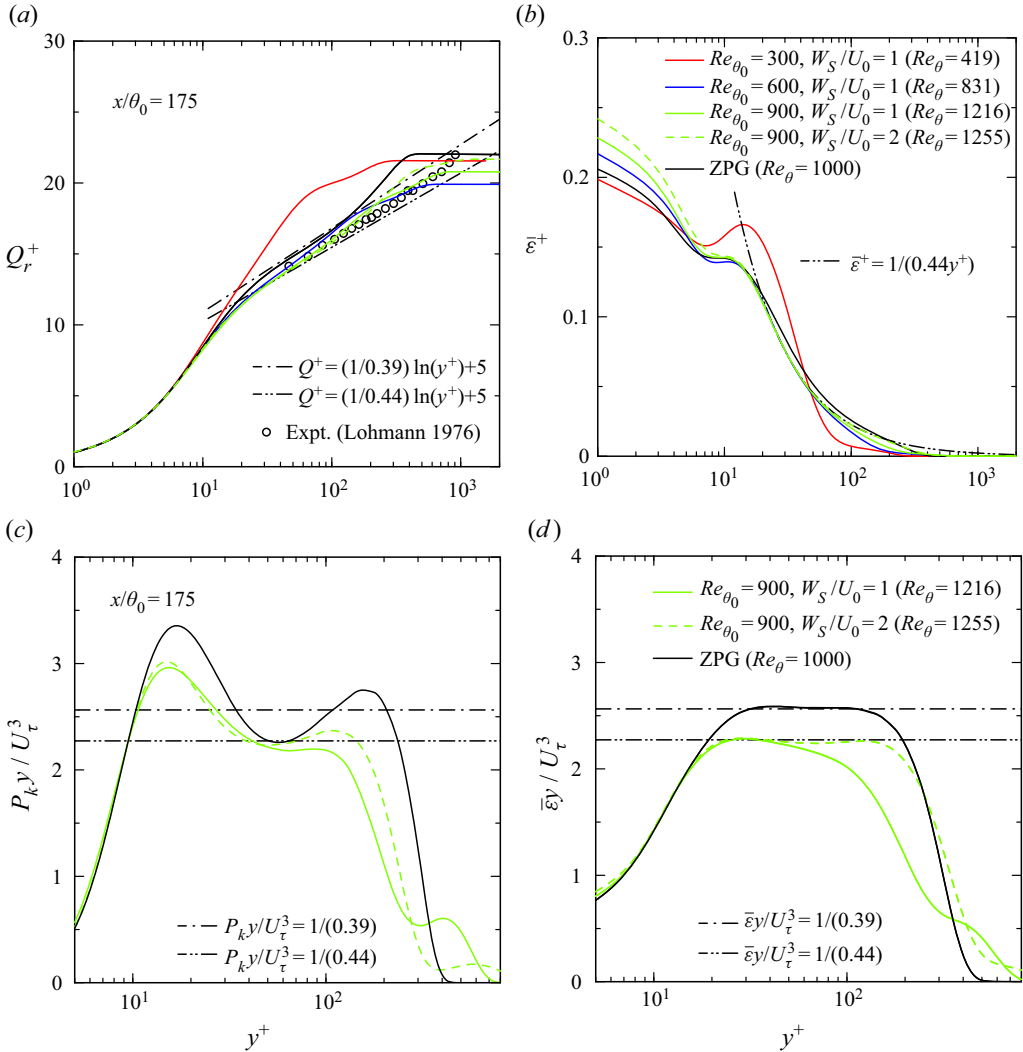
FIGURE 16. Distributions of Q_r^+ , \bar{\epsilon}^+ , P_k y / U_\tau^3 and \bar{\epsilon} y / U_\tau^3 in the 3DTBL region ( x/\theta_0 = 175 ): (a) Q_r^+ for Re_{\theta_0} = 300, 600 and 900 with W_S/U_0 = 1 and for Re_{\theta_0} = 900 with W_S/U_0 = 2 ; (b) \bar{\epsilon}^+ for Re_{\theta_0} = 300, 600 and 900 with W_S/U_0 = 1 and for Re_{\theta_0} = 900 with W_S/U_0 = 2 ; (c) P_k y / U_\tau^3 for Re_{\theta_0} = 900 with W_S/U_0 = 1 and 2 ; and (d) \bar{\epsilon} y / U_\tau^3 for Re_{\theta_0} = 900 with W_S/U_0 = 1 and 2 . The data shown have been obtained with L_{x, W_S} = 100\theta_0 . Also plotted for comparison are the DNS data of a ZPG 2DTBL for Re_\theta = 1000 obtained in the present work.
