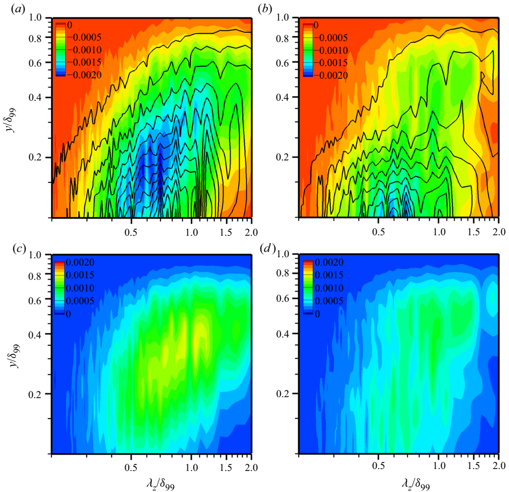
FIGURE 19. Contours in the \lambda_z - y plane of normalized premultiplied spanwise u spectra k_z\phi_{uu}(k_z) , uv co-spectra k_zCo_{uv}(k_z) and weighted uv co-spectra -4k_z(y/\delta_{99})Co_{uv}(k_z)(1 - y/\delta_{99}) in the 2DTBL and 3DTBL regions ( x/\theta_0 = 50 and 175 ) for Re_{\theta_0} = 300 with W_S/U_0 = 1 : (a) k_z\phi_{uu}(k_z)/U_0^2 (line) and k_zCo_{uv}(k_z)/U_0^2 (colour) at x/\theta_0 = 50 ; (b) k_z\phi_{uu}(k_z)/U_0^2 (line) and k_zCo_{uv}(k_z)/U_0^2 (colour) at x/\theta_0 = 175 ; (c) -4k_z(y/\delta_{99})Co_{uv}(k_z)(1 - y/\delta_{99})/U_0^2 at x/\theta_0 = 50 ; and (d) -4k_z(y/\delta_{99})Co_{uv}(k_z)(1 - y/\delta_{99})/U_0^2 at x/\theta_0 = 175 . The averaging is based on a time period t^+ \approx 2332 . The data shown have been obtained with L_x, W_S = 100\theta_0 .
