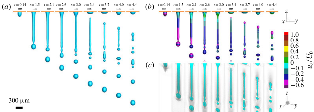
FIGURE 12. (a) Sequential images of the simulation of water injected through a 300\ \mu\text{m} hole at an exponentially slowing injection speed. (b) Sequential images as in (a) where the colour indicates u_z/U_0 , with u_z the velocity component in the z -direction and U_0 the injection speed at t = 0 ms. Even though there is much stretching before detachment, after detachment the velocities are relatively equal over the length of the ligament. This agrees with experimental results, where sequential images of the detached ligaments show very little contraction (see figures 7 and 8). (c) Velocity vectors of the middle plane of the computational domain for both liquid and air (vapour). There is a layer of air moving with the jet, that at first has a gradient in the z -direction, but at detachment becomes homogeneous.
