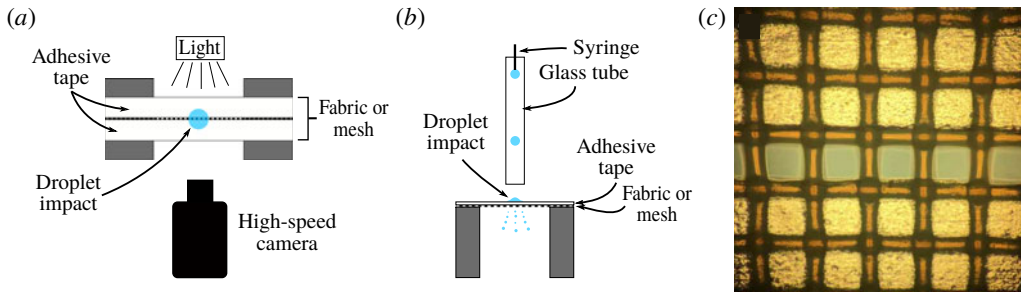
FIGURE 1. (Colour online) Schematic top (a) and side (b) views of the set-up (not to scale). A droplet (blue) impacts the middle of a fabric or mesh mounted onto two metal pillars. The tension in the mesh can be changed to alter the rigidity of the pores under study. Two pieces of adhesive tape are applied to the mesh to leave only a single row of pores open. For experiments on a full mesh, these tapes are removed. Droplet impact is filmed with a high-speed camera (around 8000 f.p.s.) with back lighting. Droplets are produced by a blunt syringe needle, and travel through a glass tube, to ensure they fall on exactly the same spot every time. (c) Microscope picture of the fabric with one row of pores left open by taping the other holes closed. Diameter of the holes is 150 \mu\text{m} .
