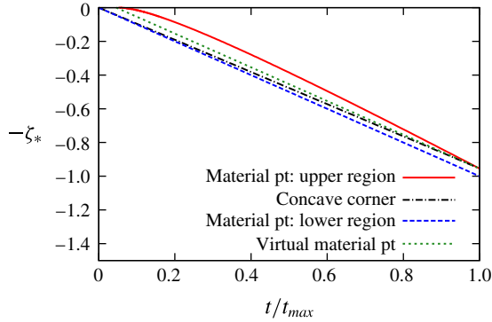
FIGURE 7. (Colour online) Plot of rescaled vertical location -\zeta_* versus rescaled time t/t_{max} representing the vertical trajectory executed by a material point in the upper region of the solution domain (see (A 3)). In addition we plot, as functions of t/t_{max} , the trajectory of the concave corner -\zeta_{*,cross} (which separates the upper and lower regions at any given time; see (A 4)), the trajectory of the material point that was originally at the top of the lower region of the solution domain -\zeta_{*,lower} (see (A 5)), and the trajectory of a ‘virtual’ material point -\zeta_{*,virtual} , which initially is in the upper region (but which moves at a speed applicable to material points in the lower region), and which is only extracted from the concave corner so as to enter the lower region at time t = t_{max} (see (A 6)).
