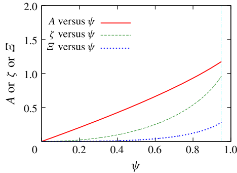
FIGURE 5. (Colour online) Solutions (corresponding to the upper region of the solution domain) obtained from the integro-differential equation for A versus \psi and \zeta versus \psi and E versus \psi , with A being rescaled angle through which the front turns, \psi being a measure of time that a given material point has been on the front (relative to total time elapsed), \zeta being rescaled vertical distance, and E being rescaled horizontal distance. The domain has been divided into 1000 intervals. The vertical line indicates where matching is achieved with the lower region of the solution domain (which occurs when \psi equals 0.948, and the solution of the integro-differential is stopped at this point).
