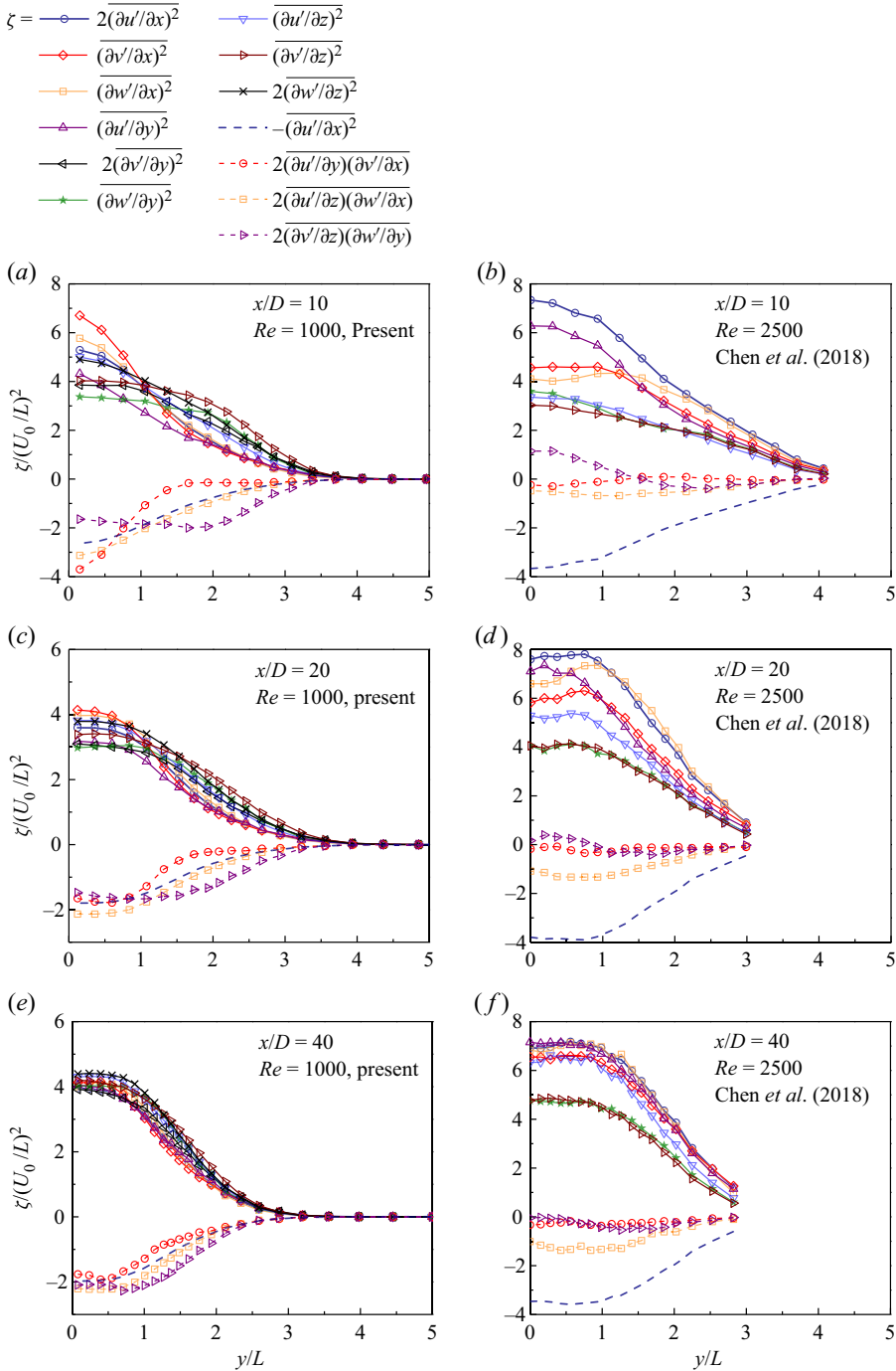
Figure 13. Transverse distributions of the 12 velocity derivative terms (denoted \zeta ) constituting the total dissipation rate: (a) x/D = 10 , Re = 1000 (present), (b) x/D = 10 , Re = 2500 (Chen et al. 2018), (c) x/D = 20 , Re = 1000 (present), (d) x/D = 20 , Re = 2500 (Chen et al. 2018), (e) x/D = 40 , Re = 1000 (present) and (f) x/D = 40 , Re = 2500 (Chen et al. 2018).
