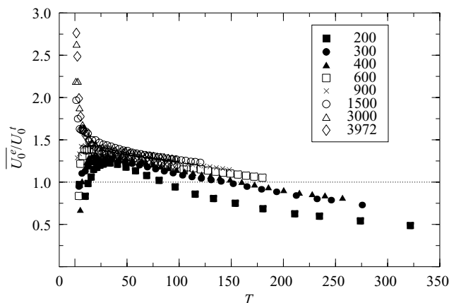
FIGURE 9. The ratio of the measured non-dimensional current mean velocity \overline{U_0^e} and the predicted velocity U_0^i = 0.75 , as a function of T . The numbers in the key are the values of q_0 in \text{cm}^3 \text{s}^{-1} .
