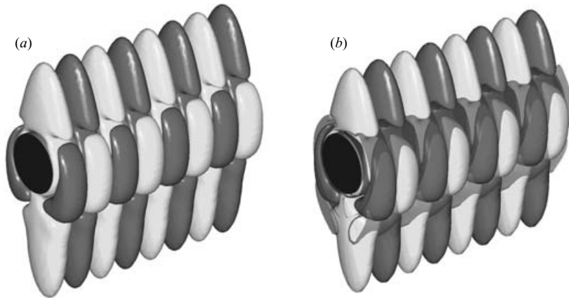
FIGURE 15. Instantaneous vorticity isosurfaces for the regime B instability at ( \beta = 80 , KC = 2.58 , k = 5.88 ), showing (a) the Floquet mode and (b) DNS result. Four spanwise repetitions are represented, at the instant when the cylinder is at y_{\max} . The solid isosurfaces show y -component vorticity of equal magnitude but opposite signs, while additionally in (b) translucent isosurfaces show z -component vorticity.
