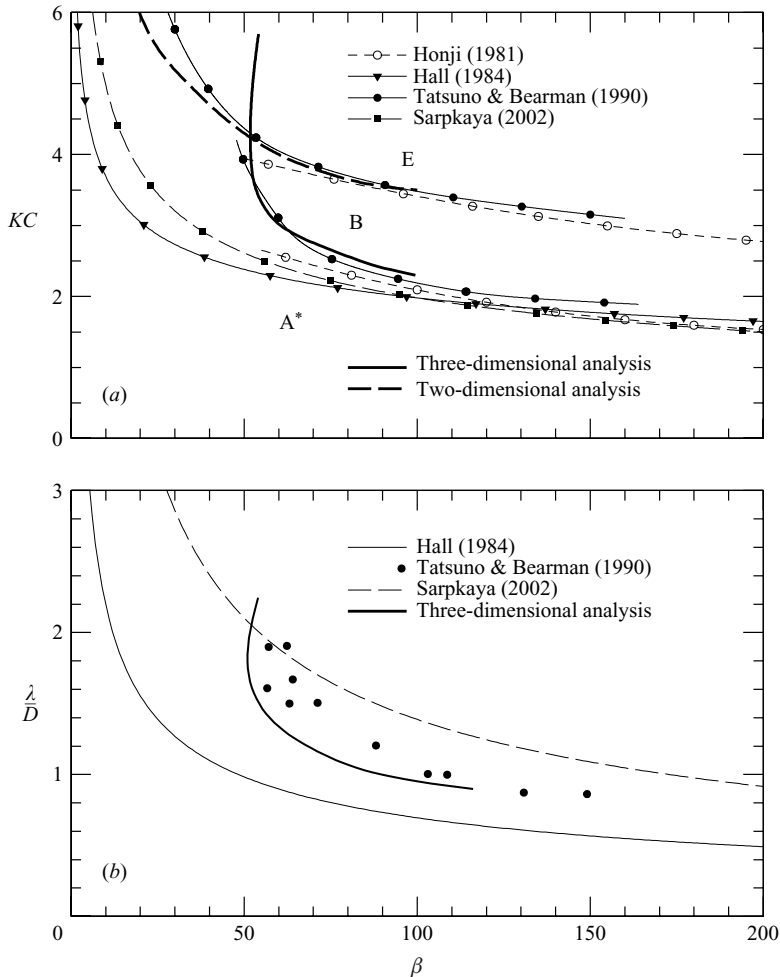
FIGURE 24. Comparison of previous results with those established via Floquet analysis. In (a), thin lines with symbols show (\beta, KC) marginal stability boundaries presented in previous experimental and theoretical studies (see legend), and thick lines those established in the present Floquet analysis. Labels A^* , B, and E are the regime names given by Tatsuno & Bearman (1990). In (b), lines and symbols show wavelengths of the corresponding three-dimensional instabilities.
