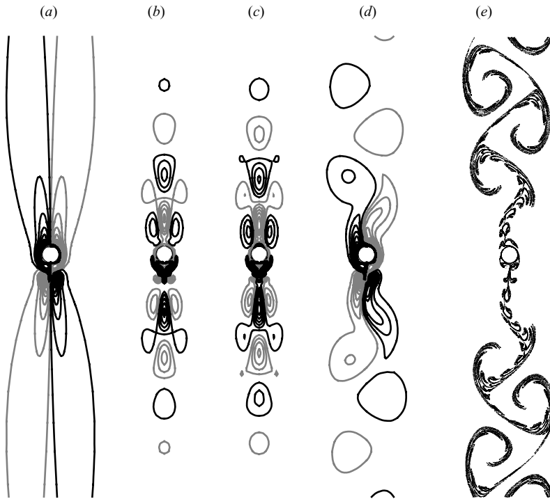
FIGURE 8. Flows of two-dimensional quasi-periodic regime QP, computed at ( \beta=40 , KC=4.7 ): (a) instantaneous vorticity contours for the basic state, with the cylinder at y=y_{\max} ; (b, c) vorticity contours of the real and imaginary parts of the Floquet eigenfunction at the same phase of the motion cycle; (d) instantaneous vorticity contours obtained from two-dimensional DNS, again at y=y_{\max} ; (e) computed positions of massless particles advected from close to the cylinder.
