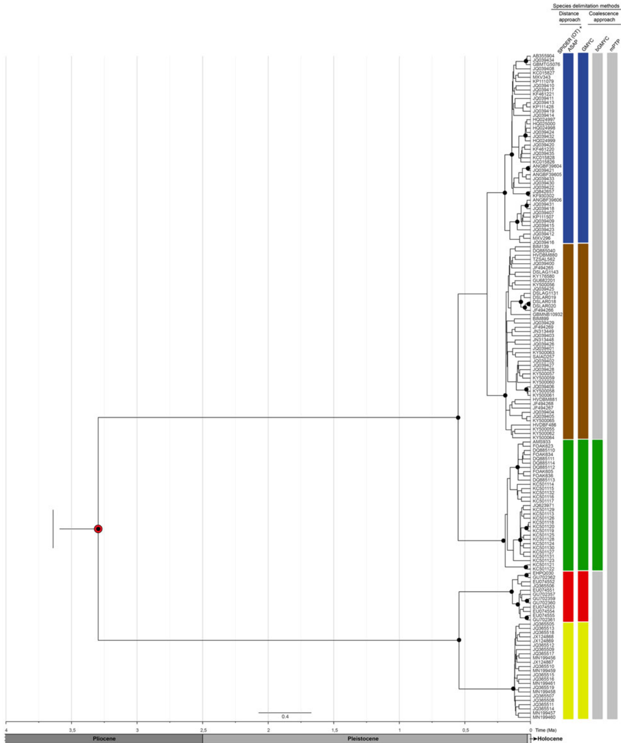
Fig. 2. Bayesian inference calibrated topology of Pomatomus saltatrix based on COI sequences and species delimitation approaches based on distance (SPIDER and ASAP) and coalescence (GMYC, bGMYC and mPPT) methods. The different coloured bars represent the MOTUs (for more details about MOTUs distribution, see Figure 1). The black circles represent posterior probabilities higher than 0.9. The red circle represents the calibrated node based on P. saltatrix fossil (Purdy et al. , 2001).
