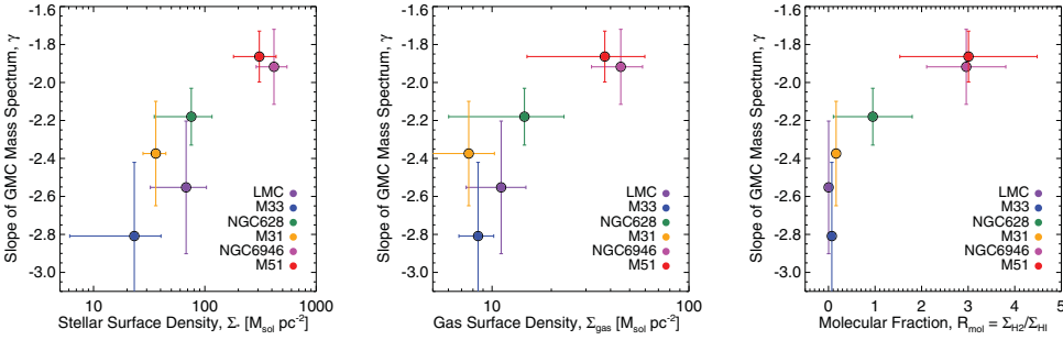
Figure 3. The power-law slope of the GMC mass distribution versus the local stellar surface density \Sigma_* (left), neutral gas surface density \Sigma_{\text{gas}} = \Sigma_{\text{HI}} + \Sigma_{\text{H}_2} (middle), and molecular fraction R_{\text{mol}} = \Sigma_{\text{H}_2}/\Sigma_{\text{H}_1} . The quantities on the x-axis are measured on 500 pc scales. The vertical error bars represent the uncertainty in the fit. The horizontal error bars indicate the 1\sigma dispersion of values within the area of the CO surveys. Taken together, the plots show that the slope of the GMC mass distribution tends to flatten as the galactic environment becomes denser and more molecule-rich.
