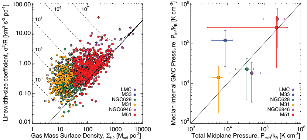
Figure 1. Left. The coefficient of the linewidth-size relation, a^2 = \sigma_v^2/R , versus the molecular gas mass surface density \Sigma_{\text{H}_2} for GMCs in M51, NGC6946, NGC628, M31, M33 and the LMC. The solid diagonal line shows the solution for simple gravitational equilibrium. The V-shaped curves represent solutions to Equation 2.1, for different values of the external pressure between P_{\text{ext}}/k_B = 10^3 and 10^7 K cm -3 . In contrast to the Larson scaling relations, the \Sigma_{\text{H}_2} values of GMCs vary by more than two orders of magnitude, and the linewidth-size coefficient increases with increasing \Sigma_{\text{H}_2} . Right. Median internal pressure of the GMCs versus an estimate of the external pressure within the region of each galaxy covered by the CO observations. The internal pressures are estimated from GMC properties and the external pressures are estimated using an expression derived by Koyama & Ostriker (2009) for the total pressure at the disk midplane (see text). The solid diagonal line indicates equality. The vertical error bars indicate the dispersion of the internal pressure estimates for individual GMCs, while the horizontal bars indicate the range of external pressures across the surveyed region.
