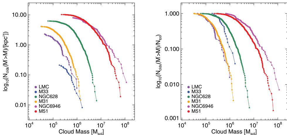
Figure 2. Cumulative mass distributions of GMCs in M51, NGC6946, NGC628, M31, M33 and the LMC, normalized by the area of the CO survey (left panel) and by the total number of identified clouds (right). The vertical offset between the curves in the left panel reflects variations in the number density of GMCs. The right panel shows that the slope of the GMC mass distribution is flatter in the denser, more massive systems (M51, NGC6946).
