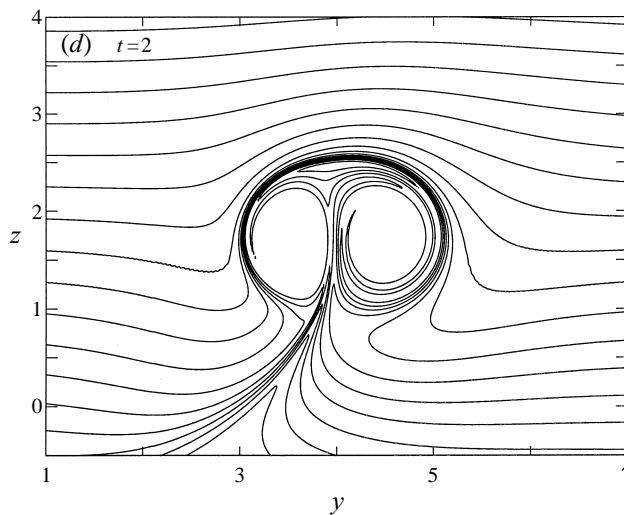
FIGURE 17( d ). Contours of ( a , b ) vorticity, ( c ) the baroclinic source of vorticity, and ( d ) density for an upwards-propagating vortex pair with Fr = 2 , Ri = 1 , and Re = 1000 . The quantities are shifted in the horizontal direction for display purposes. Primary contour levels of the vorticity are at intervals of 10, though the zero-line is not shown. Additional contour levels are shown at \pm 2 , \pm 3 , \pm 4 and \pm 5 to illustrate the distribution of vorticity with lower magnitudes, and all regions enclosed by negative contours are shaded. The contour levels of the baroclinic source are the same as for the vorticity, while the contour levels of the density are at intervals of 0.296.
