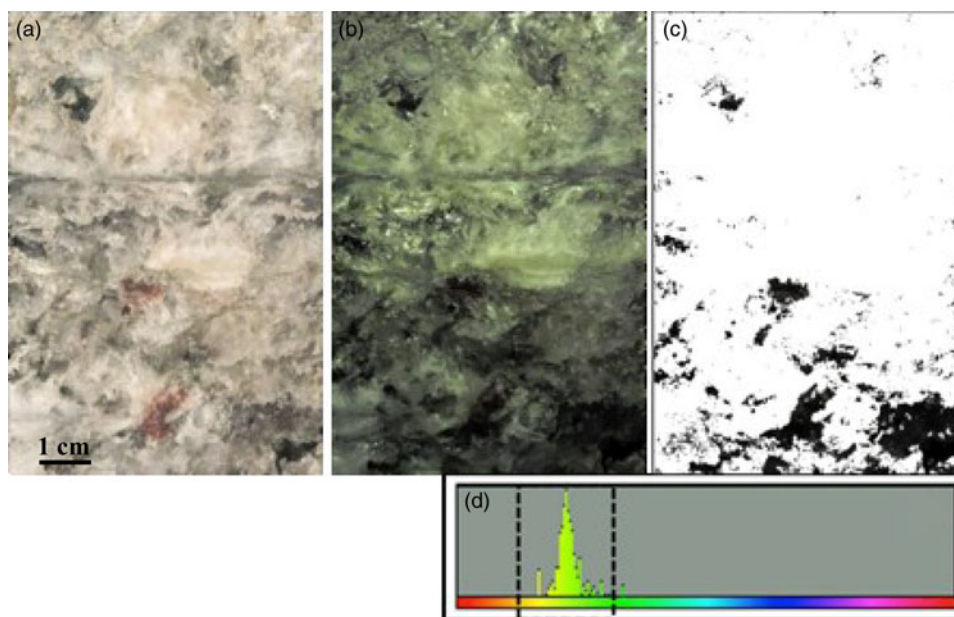
Fig. 10. Halite sample close-up area B. (a) White light CLUPI image; (b) UV-enhanced CLUPI image; (c) Non-luminescing regions (black) and luminescent regions (white) within the UV-enhanced CLUPI image B; (d) Colour histogram of 'B' showing the green fluorescence and resulting threshold boundaries for 'C'.
