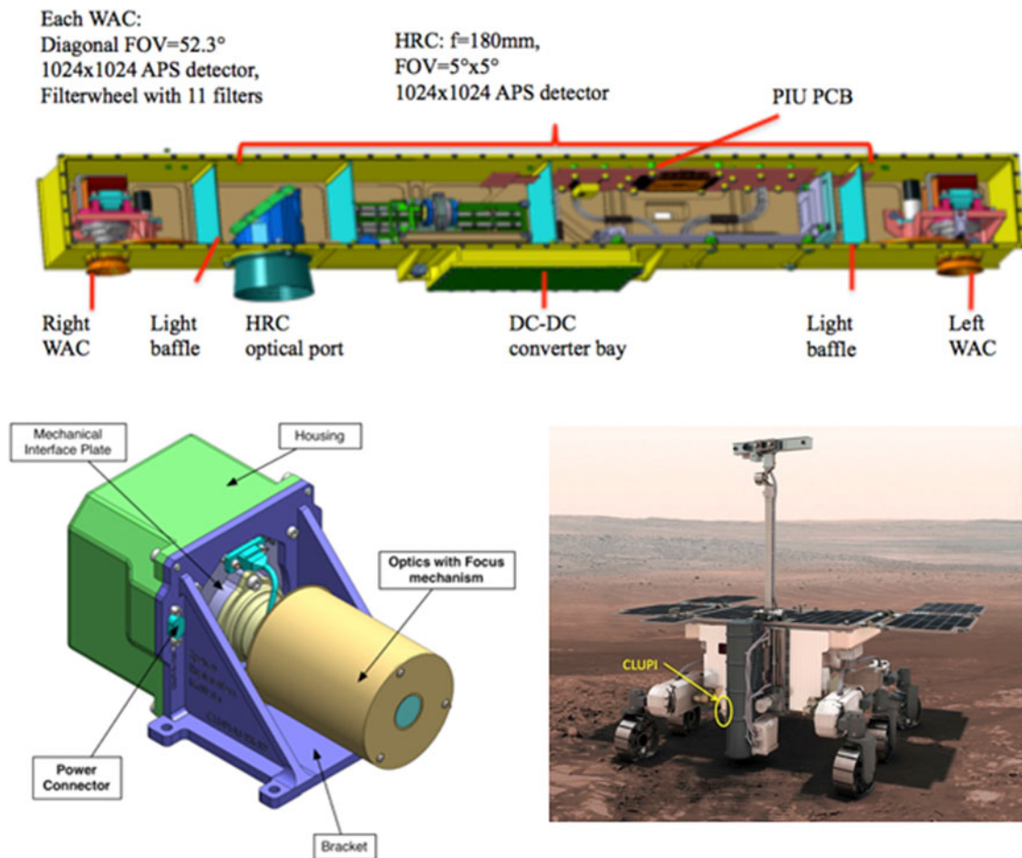
Fig. 2. Top: ExoMars PanCam optical bench. (©Mullard Space Science Laboratory). Bottom left: CAD (Computer Aided Design) of CLUPI instrument (©Space Exploration Institute). Bottom right: CLUPI and PanCam on the ExoMars rover (©ESA).
