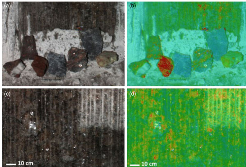
Fig. 8. Spectral parameter map overlays onto the colour background image showing the correlation of spectral properties with lithological and structural features. (a, b) Colour ROI (see Fig. 6) and associated Red/Blue ratio overlay; (c, d) colour ROI (see Fig. 6) with associated Blue/Red slope (440–660 nm), revealing the iron-rich regions (coloured red) of the exposed surface, in both the cleaned and uncleaned (top right corner) areas of the rock face.
