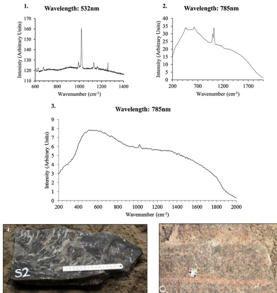
Fig. 12. Two representative Raman spectra (plots 1–2) acquired from the surface of a polyhalite sample and one from a sylvinite sample (plot 3). The data were collected with both 532 and 785 nm excitation sources. An excitation peak matches that is expected to be produced by a polyhalite mineral in both the polyhalite rock samples. The single excitation peak in the sylvinite sample (plot 3) is from the rock's small anhydrite component. Photographs 5 and 6 show the polyhalite and sylvinite samples the spectra were recorded from, respectively.
