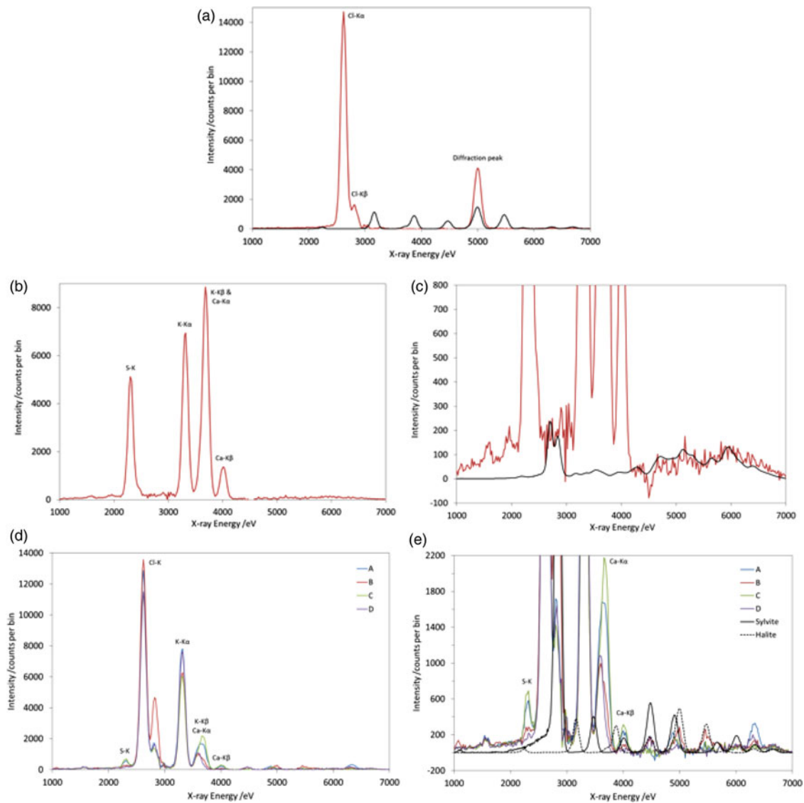
Fig. 13. Handheld XRD/XRF results; fluorescence peaks are labelled with the corresponding element. (a) Halite sample: the measured spectrum is shown in red and a diffraction-only simulation in black, illustrating the expected positions of the diffraction peaks. (b) Polyhalite sample with the fluorescence peaks are labelled. (c) As (b) but with an expanded vertical scale and with a diffraction-only simulation in black. The experimental data is negative near 4.5 keV because of imperfect background subtraction. (d) Banded potash sample measured at four different points. (e) As (d) but with an expanded vertical scale. Diffraction-only simulations are shown for sylvite (solid black) and halite (dashed black) minerals.
