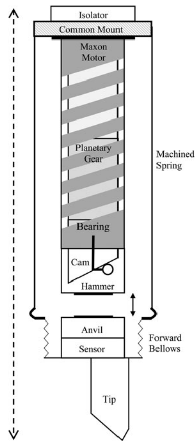
Fig. 3. Schematic of the SPLIT instrument.
