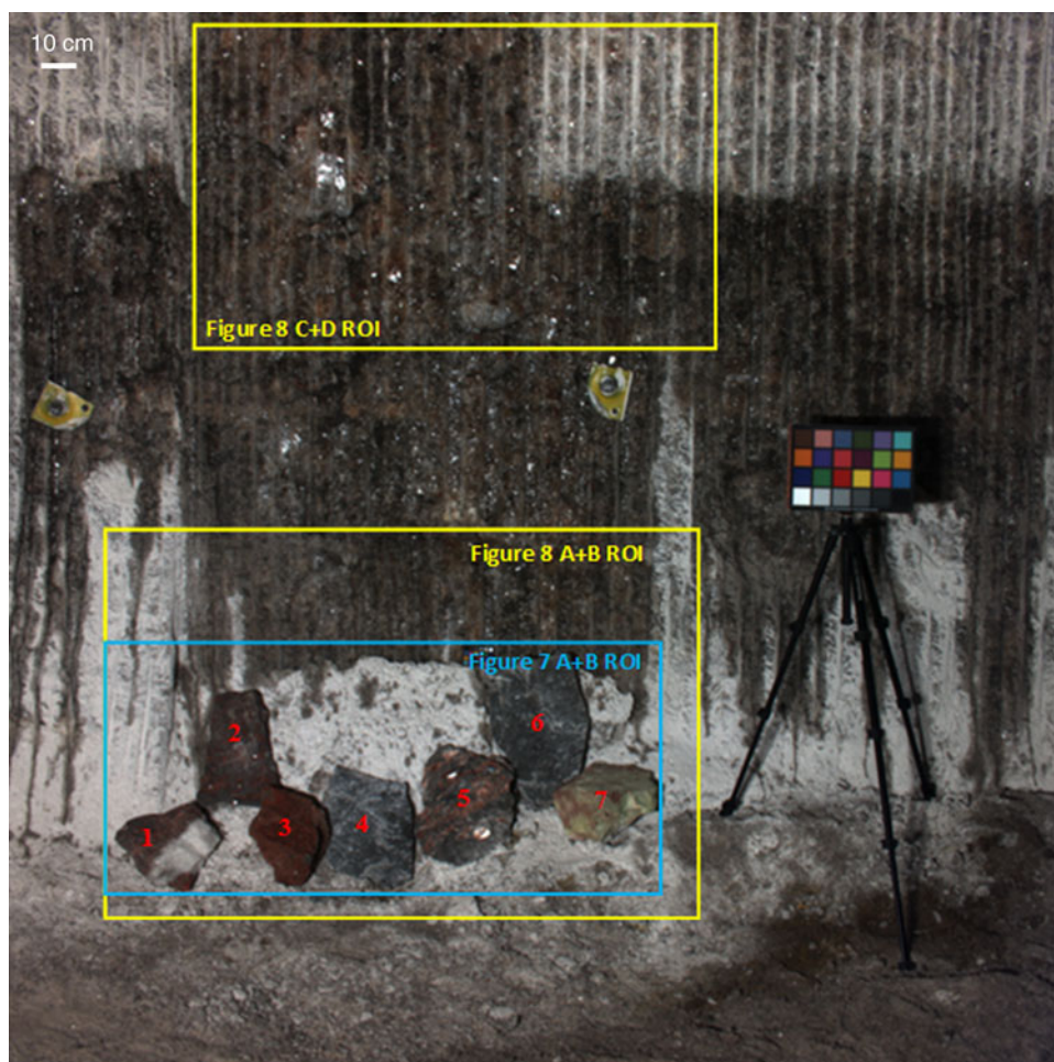
Fig. 6. Colour composite image of the test scene and target samples in Boulby mine using the broadband RGB filters. Regions of interest (ROI) for multispectral analysis are shown for Fig. 7. Image was captured from a distance of 4.85 m and illuminated by 2 \times 400 W tungsten halogen lights. Samples are: 1, 2 Sylvinitite (composed of NaCl, KCl, some \text{CaSO}_4 and insoluble clays); 3, Carnallite ( \text{KMgCl}_3 \cdot 6(\text{H}_2\text{O}) ); 4, 6, Polyhalite ( \text{K}_2\text{Ca}_2\text{Mg}(\text{SO}_4)_4 \cdot 2(\text{H}_2\text{O}) ); 5, Volkovskite ( \text{KCa}_4\text{B}_6\text{O}_8(\text{OH})_7\text{Cl} \cdot 4(\text{H}_2\text{O}) ); 7, Boracite \text{Mg}_3\text{B}_7\text{O}_{13}\text{Cl} ). The background is the halite wall of the mine.
