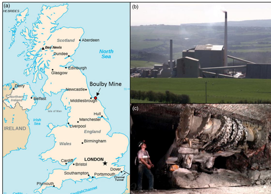
Fig. 1. (a) Location of Boulby mine (red dot). Boulby is an active Potash mine and one of the largest mines in Europe. (b) An image of the mine at the surface. (c) A typical mining scene involving the extraction of economic ore below ground.
