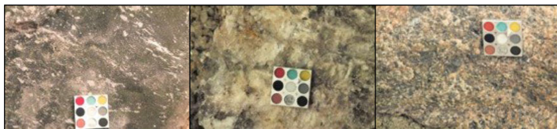
Fig. 9. Close up images of polyhalite (left), halite (centre) and sylvinite (right) taken under white light. CLUPI Calibration Target measures 2.5 \times 2.5 \text{ cm}^2 .
