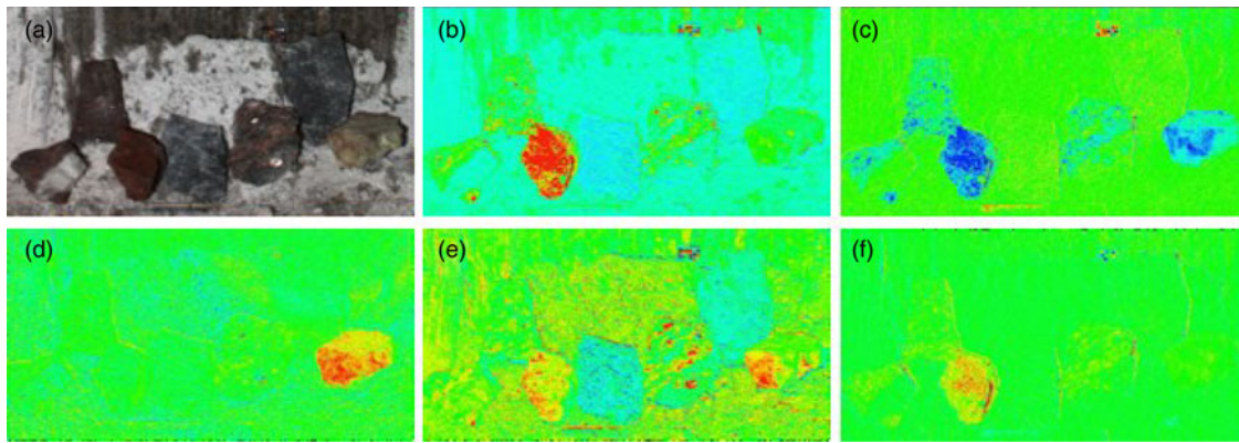
Fig. 7. Spectral parameter maps generated from AUPE-2 WAC multispectral data, demonstrating how the lithological diversity represented by the target samples in A is captured by exploiting particular wavelengths. (a) ROI from the colour composite of the scene (see Fig. 6); (b) Red/Blue ratio (671/438 nm); (c) 600 nm band depth; (d) 950–1000 nm slope; (e) Blue/Red slope (438–671 nm); (f) 532 nm band depth. Artefacts in the corners of the images are due to vignetting.
