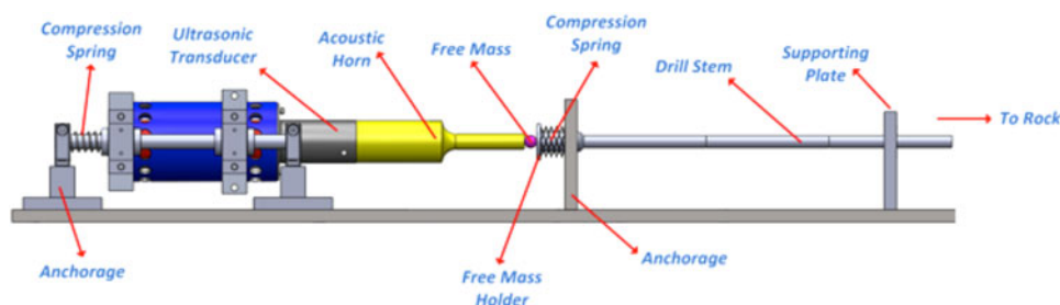
Fig. 4. Experimental setup of the percussive drilling unit.
