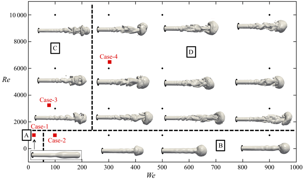
Figure 2. Regime map of the phenomenological interfacial dynamics in the Re – We space using the M2 mesh (see table 5 in Appendix A for mesh details). Four different regimes and their boundaries are identified. A snapshot of the flow corresponding to the three-dimensional representation of the interface for each simulated point (i.e. black marker) is shown. The red squares refer to the cases presented in table 2.
