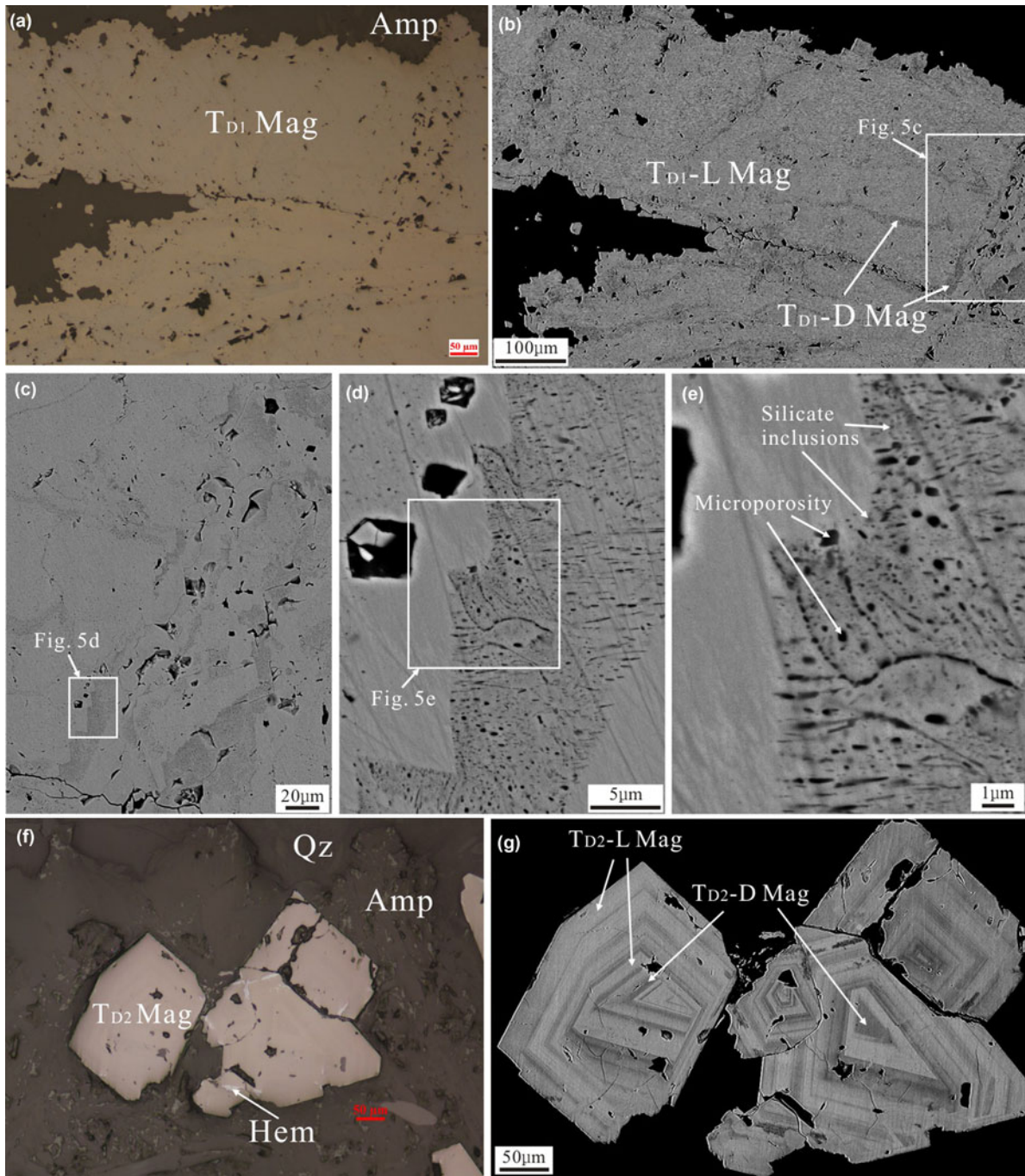
Fig. 4. Photomicrographs ( a, f ) and BSE images ( b–e, g ) of the Duotoushan magnetite. ( a ) Photomicrograph of platy magnetite ( T_{D1} Mag), which shows different zones. The T_{D1-L} magnetite is the bright domain. The T_{D1-D} magnetite is the dark domain with abundant microporosity and silicate inclusions. ( f ) Photomicrograph of granular magnetite ( T_{D2} Mag). ( g ) BSE image of platy magnetite, which shows obvious oscillatory zones. Mineral abbreviations (from Whitney and Evans, 2010): Mag: magnetite, Amp: amphibole; Qz: quartz; Hem: hematite.
