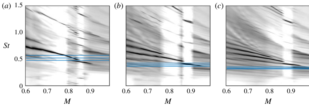
FIGURE 14. Low-frequency resonance cutoff, shown by horizontal blue lines, from (a) to (c) |R_1R_2| = 0.002, 0.004 and 0.008 .
