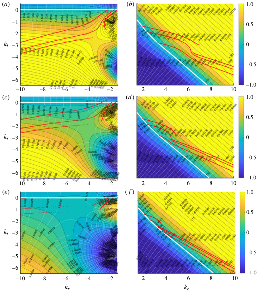
FIGURE 21. Vortex-sheet solutions, \omega(k) . The colour map shows \omega_i ; white isocontours show St = \omega_r/2\pi . Red dots indicate k^- (left plot) and k^+ (right plot) modes satisfying the resonance amplitude constraint (B 8). From top to bottom: M = 0.6, 0.7 and 0.8 . Solid white lines show neutral-mode model branches ( \omega_i = 0 ).
