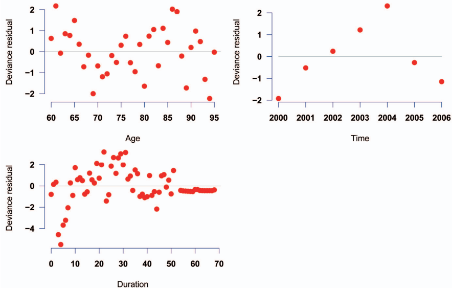
Figure 6. Deviance residuals plotted against: (1) age; (2) calendar time; and (3) duration since pension commencement
