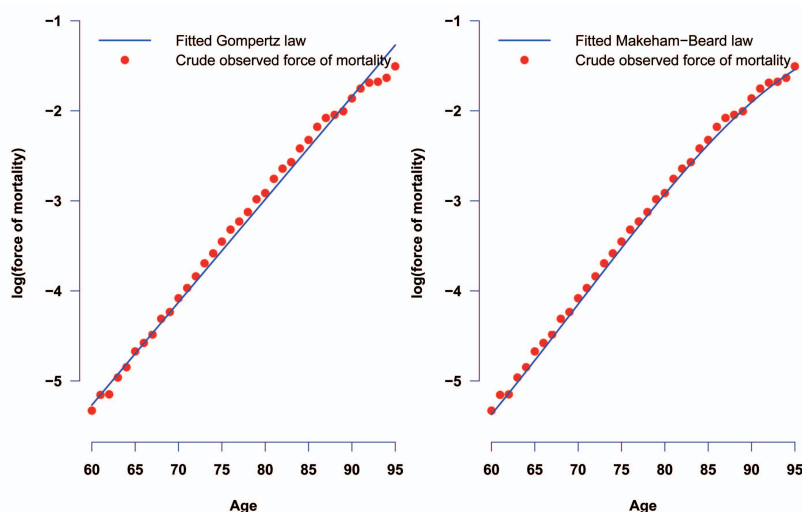
Figure 4. Comparison of Gompertz and Makeham-Beard models for age only
