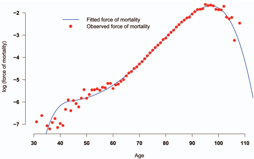
Figure 2. Force of mortality for pensioners between ages 30 and 110
