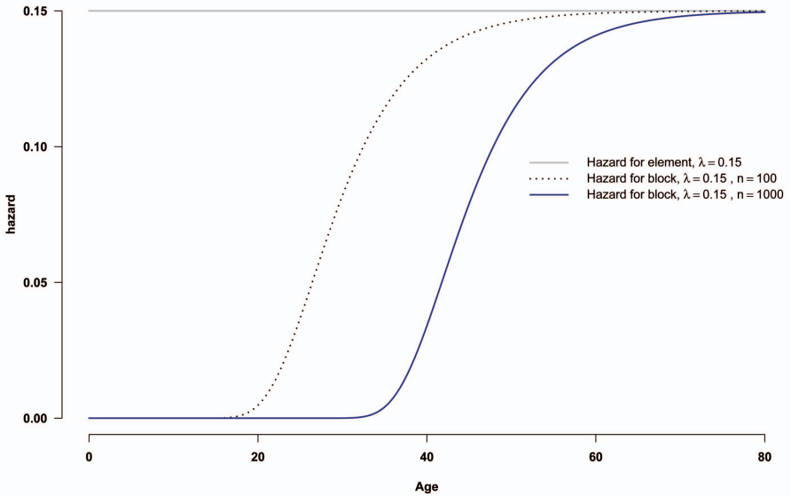
Figure 10. Diagram illustrating hazard functions for elements and blocks
