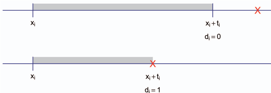
Figure 1. Diagram of survival-model setup
