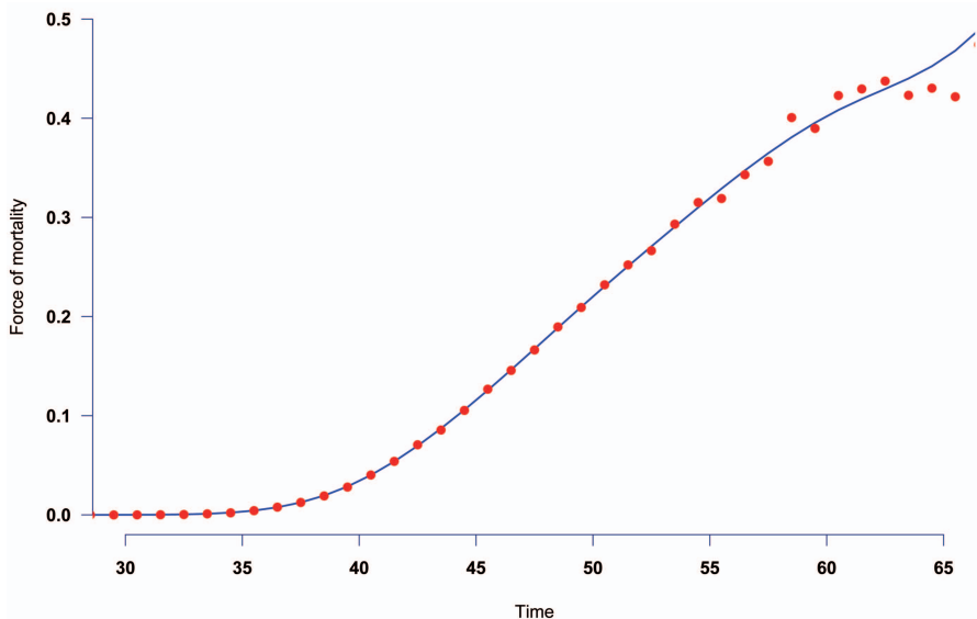
Figure 13. Force of mortality in one million simulations of ruin
