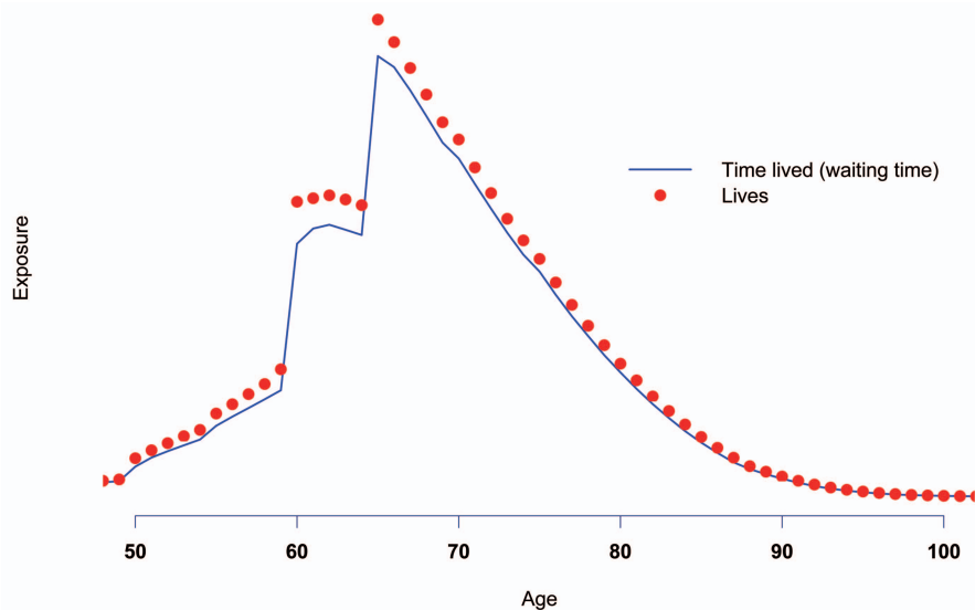
Figure 3. Distribution of lives and exposure
