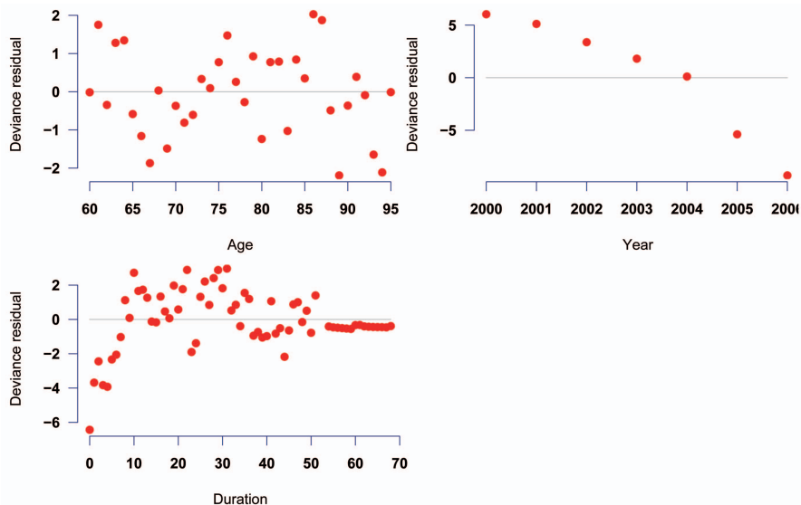
Figure 5. Deviance residuals plotted against: (1) age; (2) calendar time; and (3) duration since pension commencement
