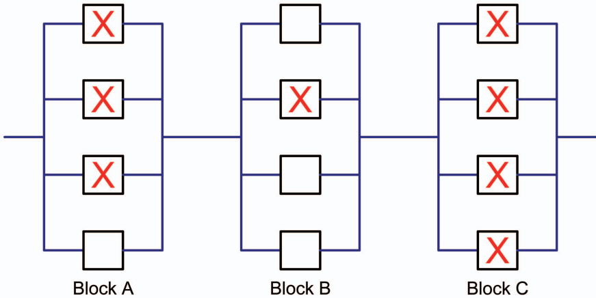
Figure 11. Diagram illustrating a system with redundancy
