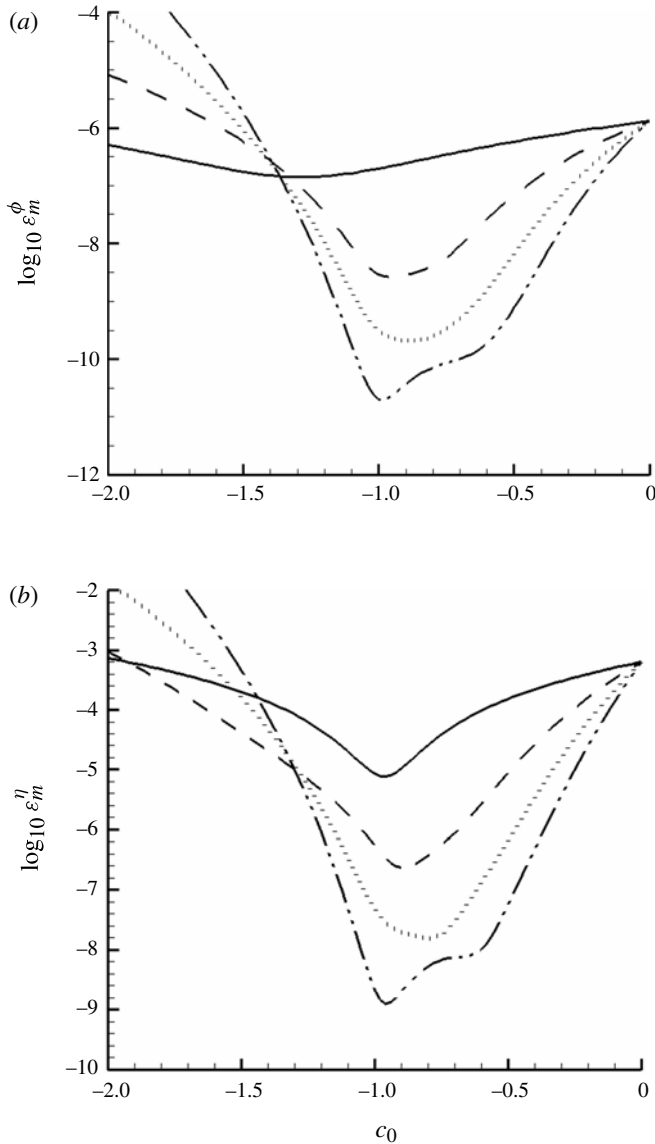
FIGURE 2. Residual squares of \log_{10} \epsilon_m^\phi and \log_{10} \epsilon_m^\eta versus c_0 for (4.1) with \epsilon = 1.0003 , k_2/k_1 = 0.913835 and k_2 d = 3\pi/5 when A_0 = -0.061834 , B_0 = 0.043603 and C_0 = -0.0866169 (corresponding to group A1). Solid line, first-order approximation; dashed line, third-order approximation; dotted line, fifth-order approximation; dash-dot-dotted line, seventh-order approximation.
