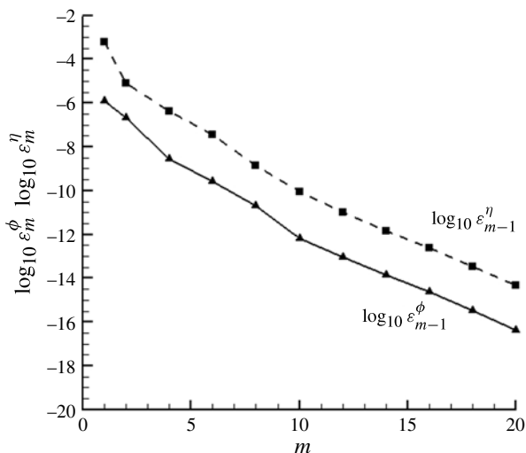
FIGURE 3. Residual squares of \log_{10}\epsilon_m^\phi and \log_{10}\epsilon_m^\eta versus the approximation order m for (4.1) with \epsilon = 1.0003 , k_2/k_1 = 0.913835 and k_2d = 3\pi/5 when A_0 = -0.061834 , B_0 = 0.043603 and C_0 = -0.0866169 (corresponding to group A1) by means of c_0 = -0.98 . Solid line, \log_{10}\epsilon_m^\phi ; dashed line, \log_{10}\epsilon_m^\eta .
