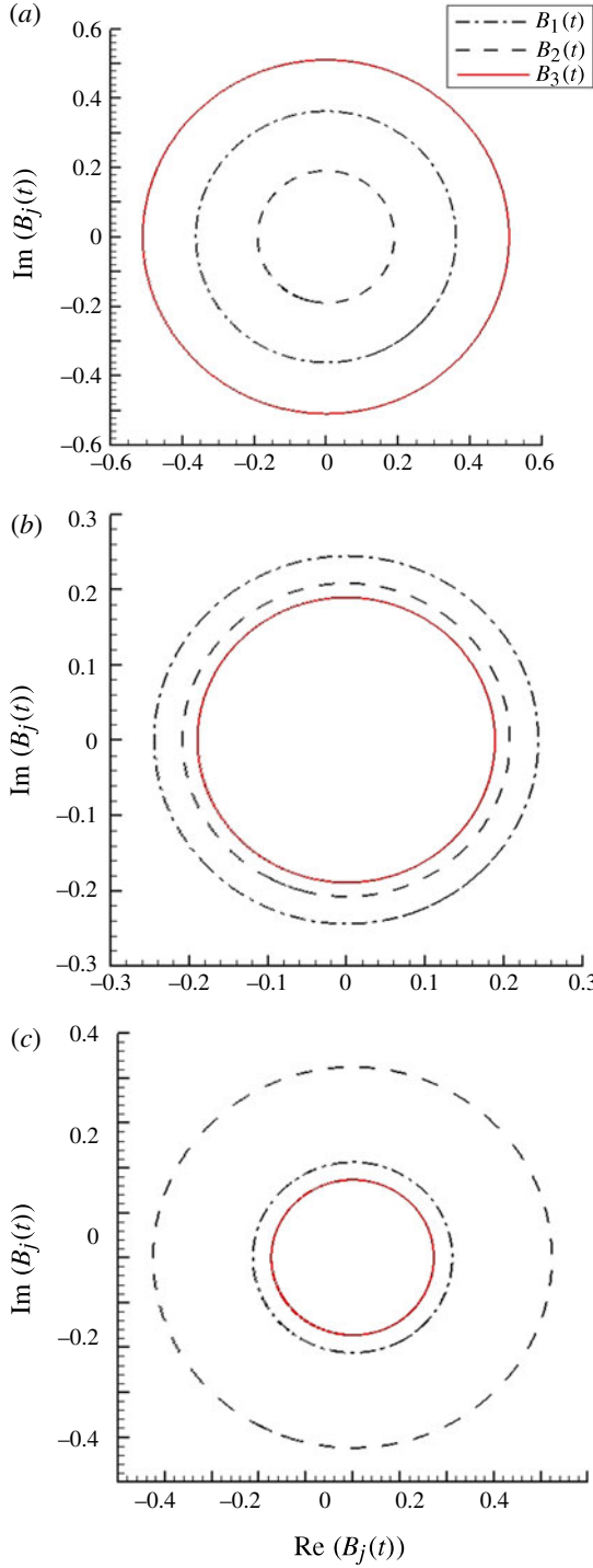
FIGURE 7. (Colour online) Time-independent norm |B_j(t)| of (B 6)–(B 8) for (4.1) with \epsilon = 1.0003 , k_2d = 3\pi/5 and k_2/k_1 = 1.11165 . (a) Group ZB1, (b) group ZB2, (c) group ZB3. Dash-dotted line, B_1(t) ; dashed line, B_2(t) ; solid line, B_3(t) .
