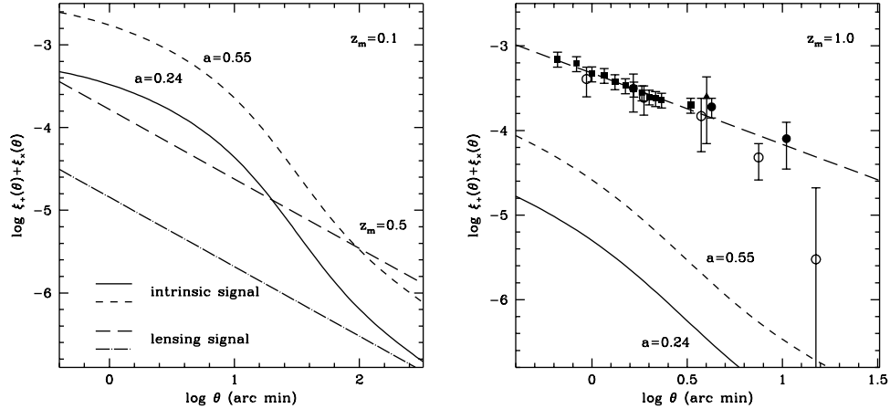
Figure 1 The intrinsic correlation signal versus the predictions from weak lensing and current observations. Left panel: predictions for a shallower survey such as SDSS and 2dF with z_m = 0.1 . The intrinsic signal is plotted for two values of a , and the theoretical prediction for weak lensing is the long-dashed line (for z_m = 0.1 ) and dotted-long-dashed (for z_m = 0.5 ). The lensing prediction for z_m = 0.1 is extrapolated from the Jain & Seljak (1997) fit beyond the stated range of validity. For such low redshifts the intrinsic signal dominates on most scales. Right panel: \xi_+(\theta) + \xi_\times(\theta) the intrinsic signal for z_m = 1 , compared to the measured shear correlation function. At small separations, the intrinsic signal is approximately 1% of the lensing signal. The amplitude depends on the assumed average galaxy thickness ( \alpha ) and the parameter a that describes how well the angular momentum of the galaxy is correlated with the distortion field. We plot a = 0.24 (full line) and a = 0.55 (short-dashed line) which correspond to the values inferred from the numerical simulations of Lee & Pen (2000) and Heavens, Refregier & Heymans (2000). \alpha = 0.73 corresponds to the value determined from the observed distribution of ellipticities. The data are: van Waerbeke et al. (2000) — solid squares ; Wittman et al. (2000) — filled circles ; Kaiser et al. (2000) — open circles; and Bacon et al. (2000) — filled triangle. The long-dashed line is the extrapolated theoretical prediction from Jain & Seljak (1997) computed for a \Omega_\Lambda = 0.7 galaxy cluster normalised flat universe, \sim 4.75 \times 10^{-4}(\theta/\text{arc min})^{-0.84} .
