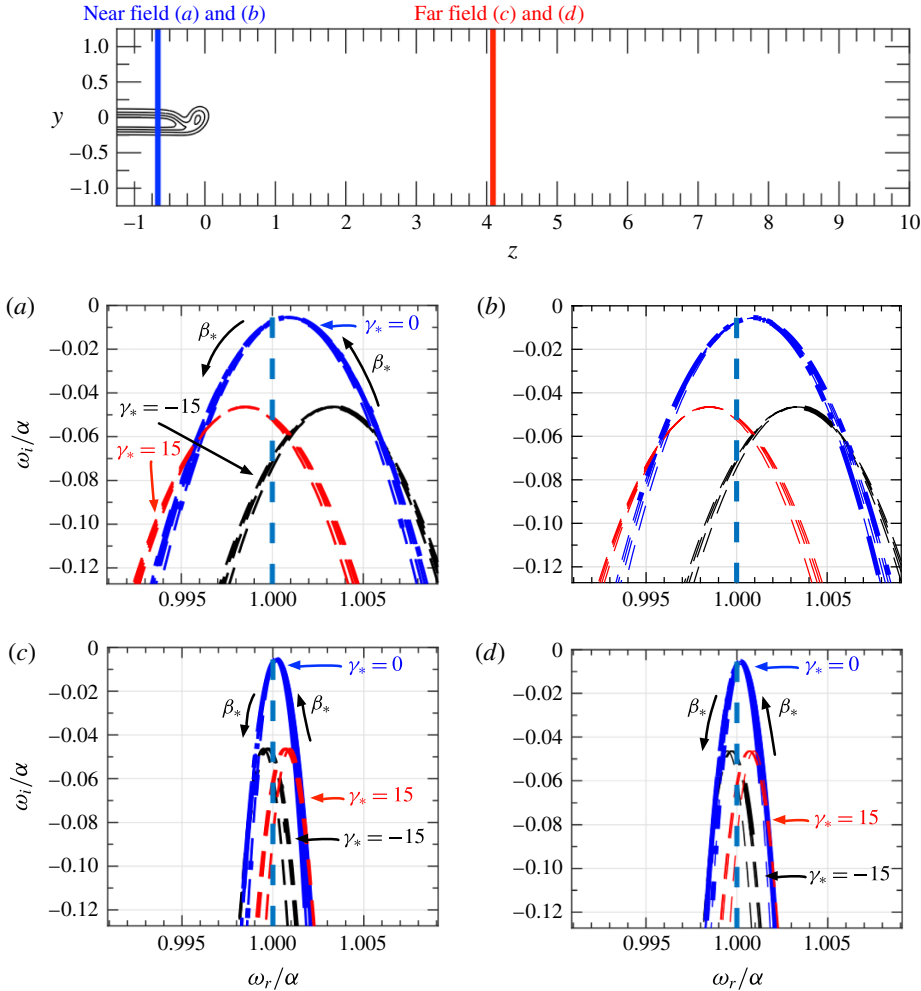
FIGURE 28. (Colour online) Symbol curves for constant z_* = -0.67 in the near field, (a) and (b), and z_* = 4.09 the far field, (c) and (d), for the first and second solutions, respectively. The line colours correspond to \gamma_*/h = -15 (black), \gamma_*/h = 0 (blue) and \gamma_*/h = 15 . The dashed lines correspond to where the twist condition is not satisfied, while the solid lines denote where the twist condition is satisfied. The top figure shows the locations of each z_* slice in the near field and far field.
