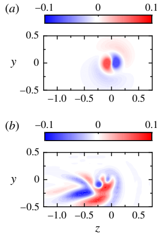
FIGURE 25. Comparison of the streamwise vorticity of the Batchelor vortex instability (a) with the bi-global vortex instability (b). Although the discrete branches align, the Batchelor vortex fails to capture the wake–vortex interaction.
