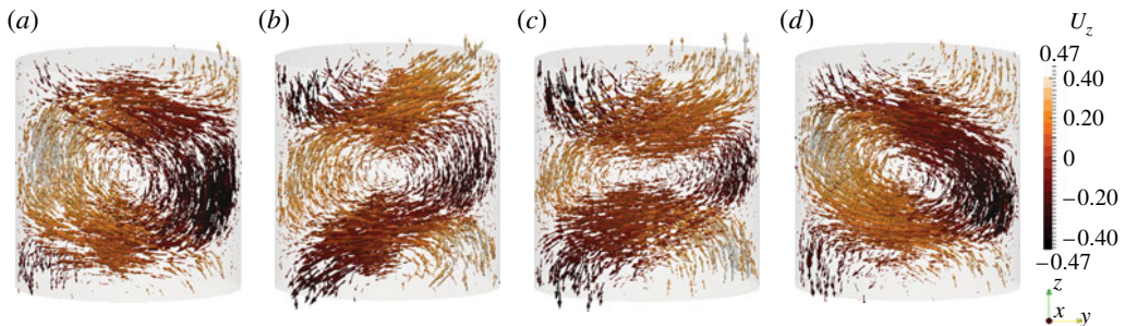
FIGURE 5. (Colour online) Periodic TB-BC, h = 2 , time-periodic state at Ha = 35 and Pm = 10^{-2} : (a) t and t + T ; (b) t + T/4 ; (c) t + T/2 ; (d) t + 3T/4 . Two pulsating vortices in phase opposition.
