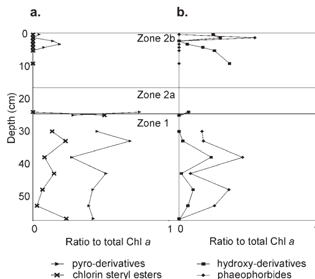
Fig. 7. Depth profiles of a. pyro-derivatives and CSEs, and b. ^{13}\text{C} -hydroxy-derivatives and Pheids relative to the total Chl a signal in the Progress Lake sediment.
