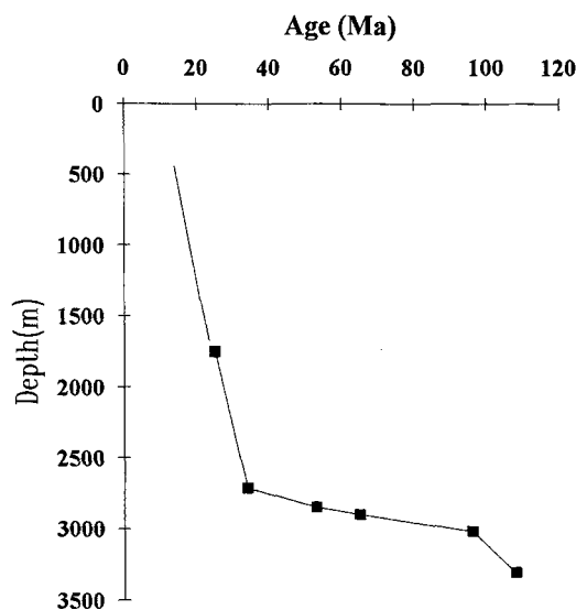
Figure 2. Sedimentation history in the well studied shown as a function of depth and age of the sediments.
