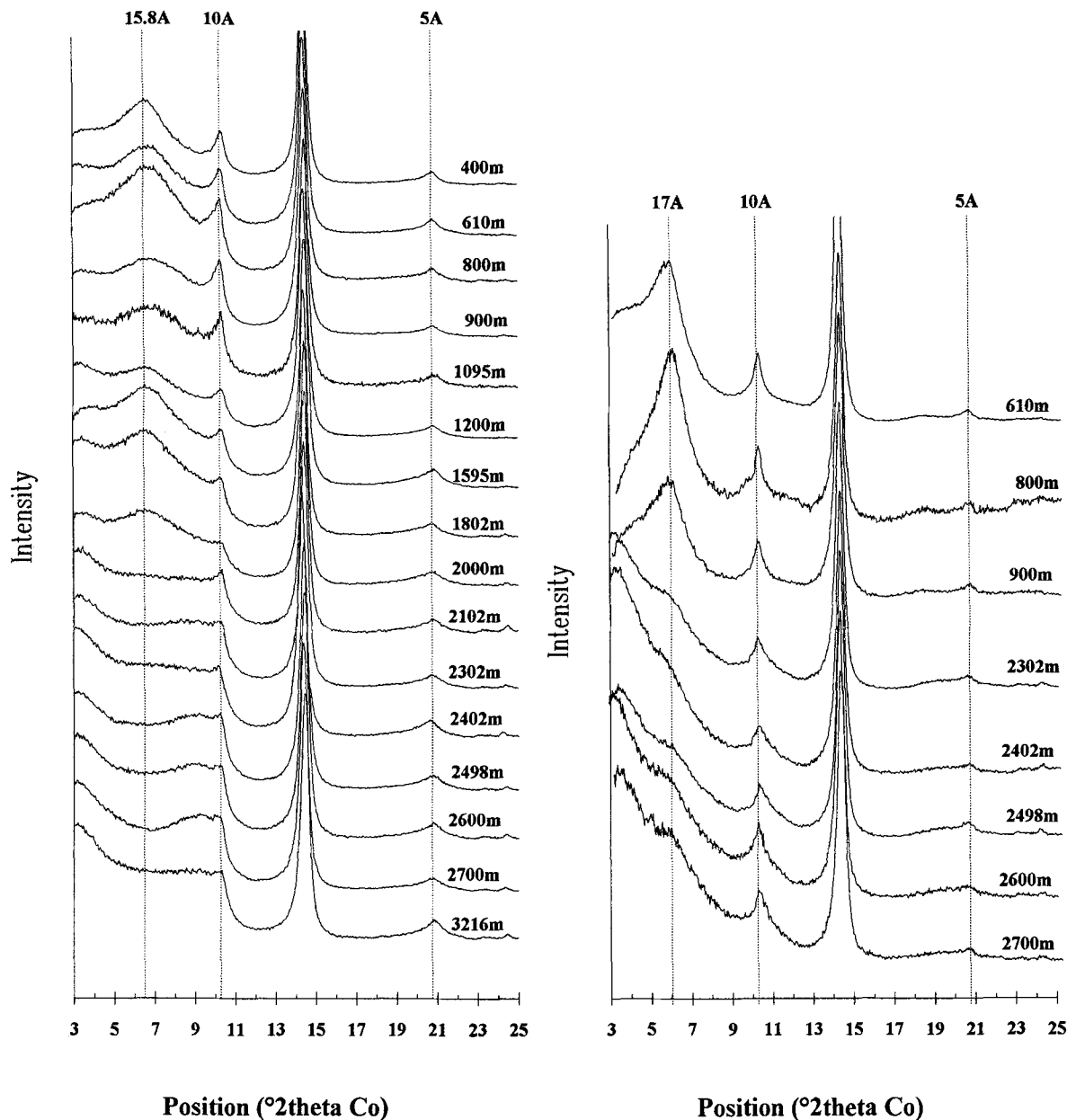
Figure 3a. Raw XRD patterns in air-dried state show the evolution of the spectra with depth in the well studied. Note the continued, very intense peak for kaolinite at 14.5 degrees. Figure 3b. Glycolated samples.
