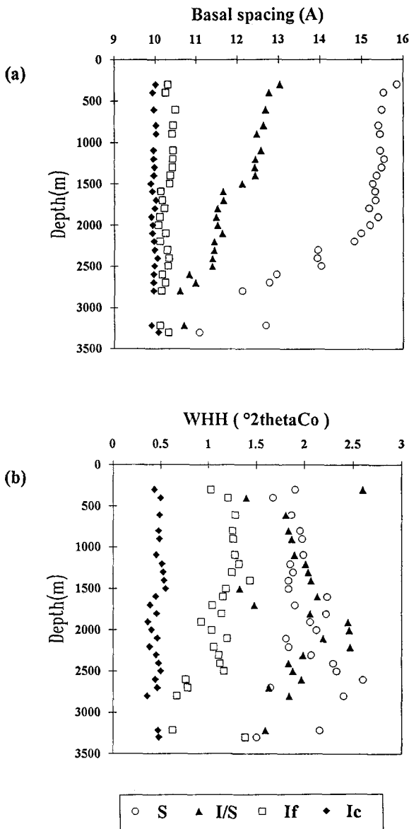
Figure 5. Plot of decomposition band position and band width at half height (WHH), for the identified phases after decomposition as a function of depth in the well. circles = smectite band, triangles = I/S band, squares = If fine-grained illite, and diamonds = Ic coarse-grained illite.
