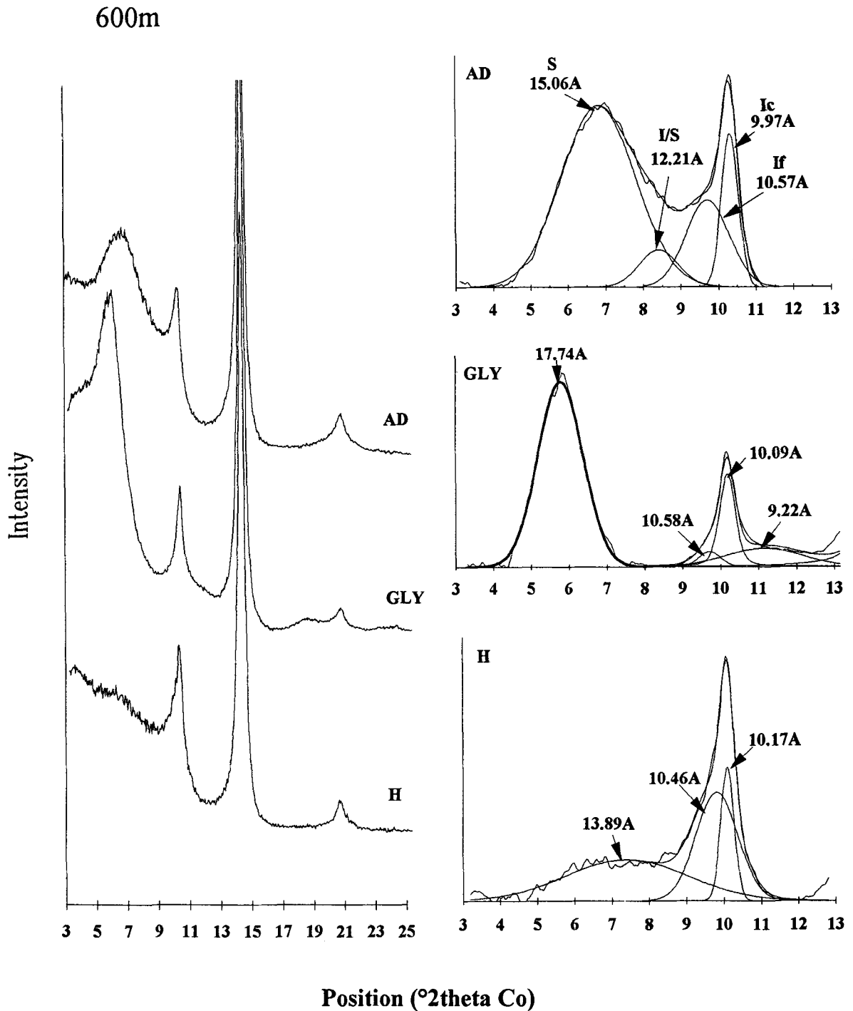
Figure 1 a–b. X-ray diffractograms (Co radiation) of two samples from the Angola well depths of 600 and 2300 m. Air dried (AD), glycolated (GLY) and samples heated (H) to 200 °C. Decomposition of the mica-smectite (001) bands is shown.
