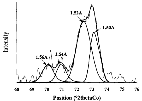
Figure 6. Decomposed spectra of the (060) region for a smectite-rich sample. Two dioctahedral band positions are apparent, one at 1.50 and the other at 1.52 Å.
