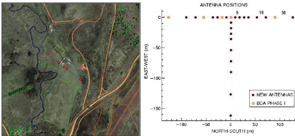
Figure 1. Aerial view of the BDA site (left) and proposed antennas configuration for BDA - Phase II (right). The red circles in the left image correspond to the antennas of BDA Phase I.
