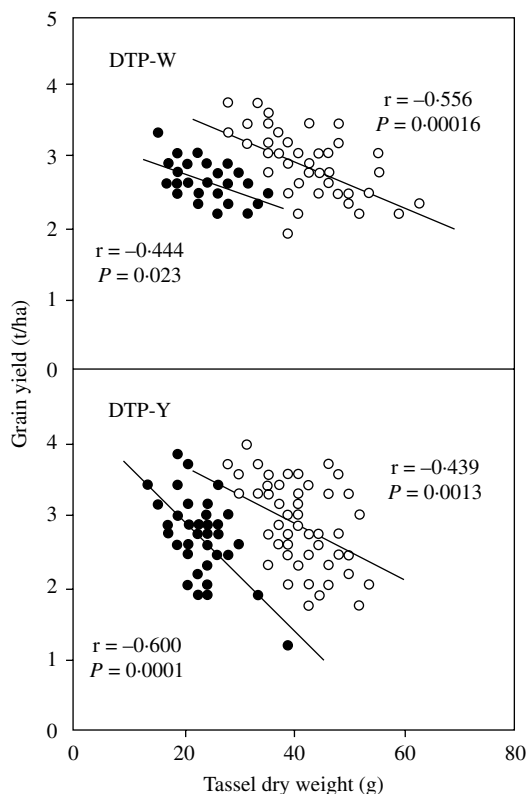
Fig. 1. Correlation between tassel dry weight and grain yield under drought conditions in DTP-W and DTP-Y hybrids in Year 1 (open circles) and Year 2 (black circles). Hybrids were grown under managed drought conditions and the tassel from five plants of each plot was removed before male flowering. Values for grain yield represents the average of three replicates of plots containing 52 well bordered plants. Each dot represents a given genotype with its mean trait values after statistical analysis. Regression lines and correlation values for Years 1 and 2 are given.
