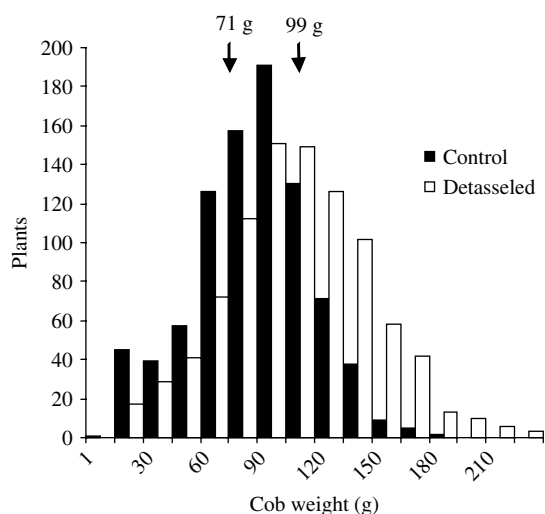
Fig. 2. Effect of detasselling on grain yield in DTPW three-ways hybrids under drought conditions in Year 2. Growing tassels were cut manually prior male flowering. Detasseled and non-detasseled control plants were harvested separately and ear weight was determined individually per plant. The histogram presents the distribution of measured ear weights of 960 plants for each type of treatment ( n = 960 ). Arrows denote the average ear weight from control (71 g) and detasseled plants (99 g).
