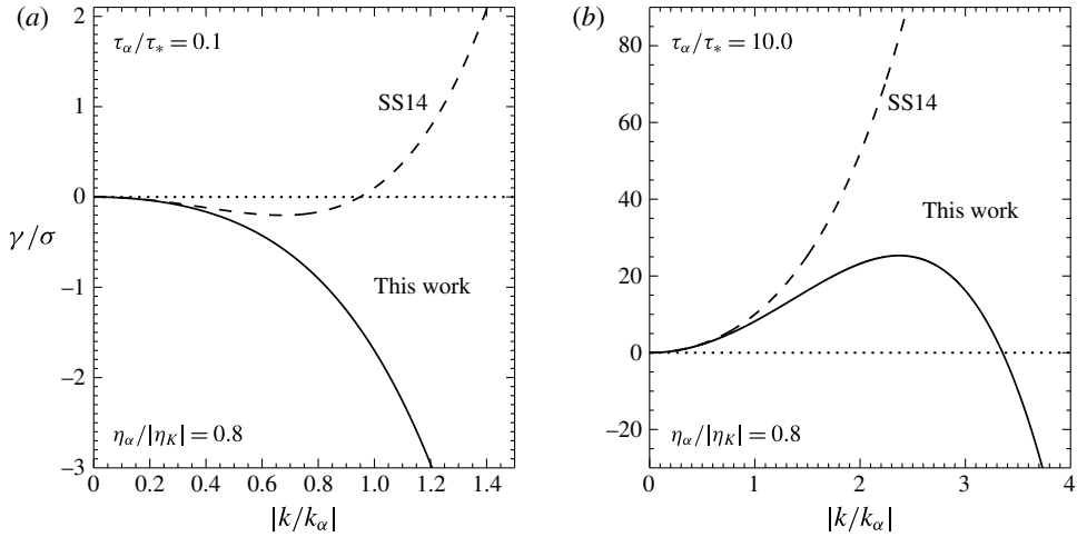
FIGURE 2. Growth rate \gamma/\sigma plotted as a function of |k/k_\alpha| for weak \alpha fluctuations; shown by solid curves. Panels (a) and (b) correspond to the case when \tau_\alpha/\tau_* = 0.1 and 10.0, respectively. Dashed curves correspond to the results of SS14.
