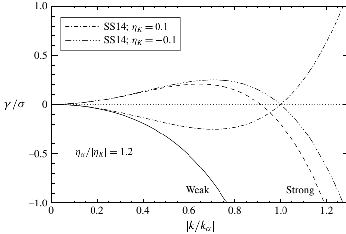
FIGURE 1. Growth rate \gamma/\sigma as a function of |k/k_\alpha| , when \mathbf{V}_M = \mathbf{0} . Weak ( \eta_K > 0 ) and strong ( \eta_K < 0 ) \alpha fluctuations correspond to solid and dashed curves, respectively. Results of SS14 are also shown; dash-dotted and triple-dot-dashed curves correspond to weak and strong \alpha fluctuations, respectively.
