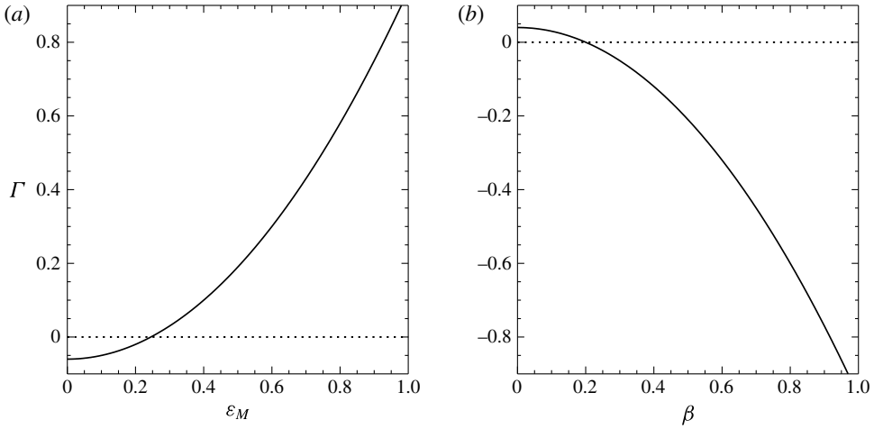
FIGURE 4. Growth rate function \Gamma plotted as a function of (a) \varepsilon_M for \beta = 0.1 , and (b) \beta for |\varepsilon_M| = 0.3 ; in both the cases, \varepsilon_K = 0.05 .
