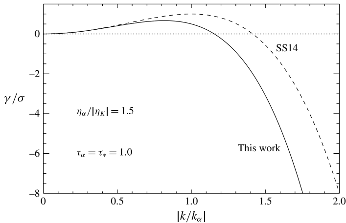
FIGURE 3. Growth rate \gamma/\sigma plotted as a function of |k/k_\alpha| for strong \alpha fluctuations; shown by solid curve. Dashed curve correspond to the results of SS14.
