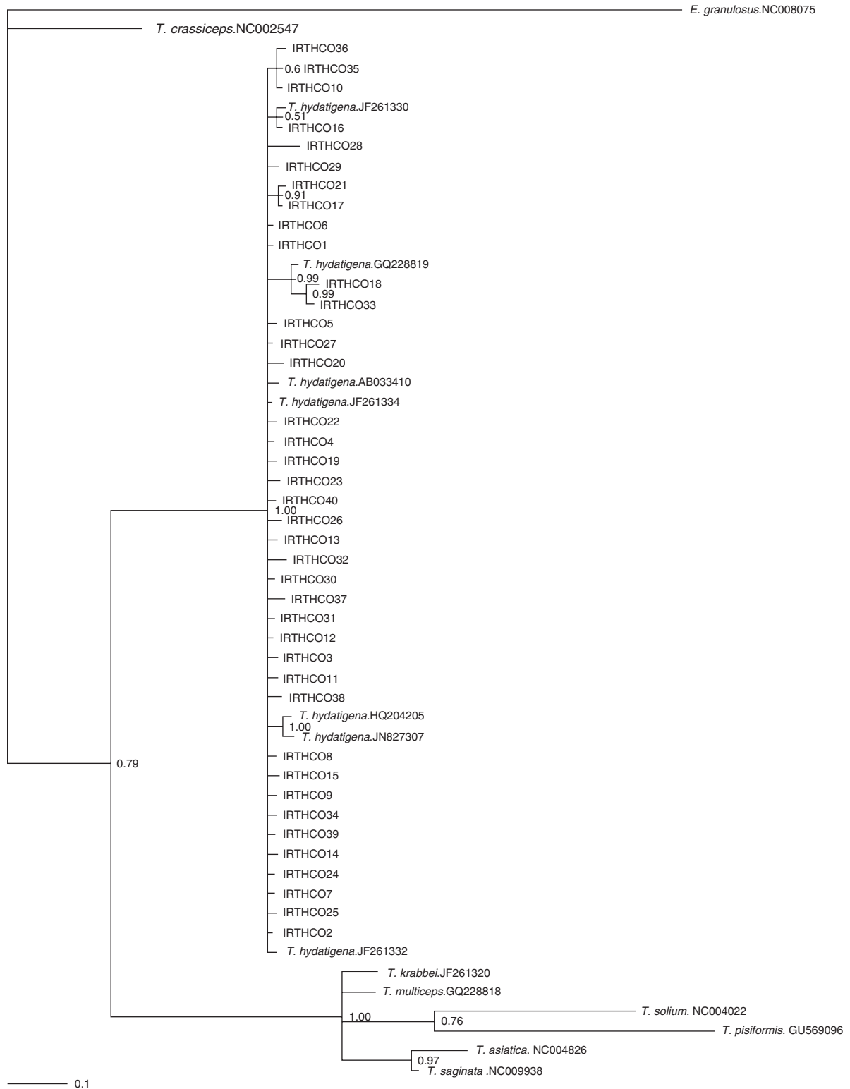
Fig. 1. Phylogenetic analyses of Taenia hydatigena isolates to show partial CO1 (390 bp) sequences; distance (% substitution per site) is shown by a scale bar and nodal support by a posterior probability (pp) value.
