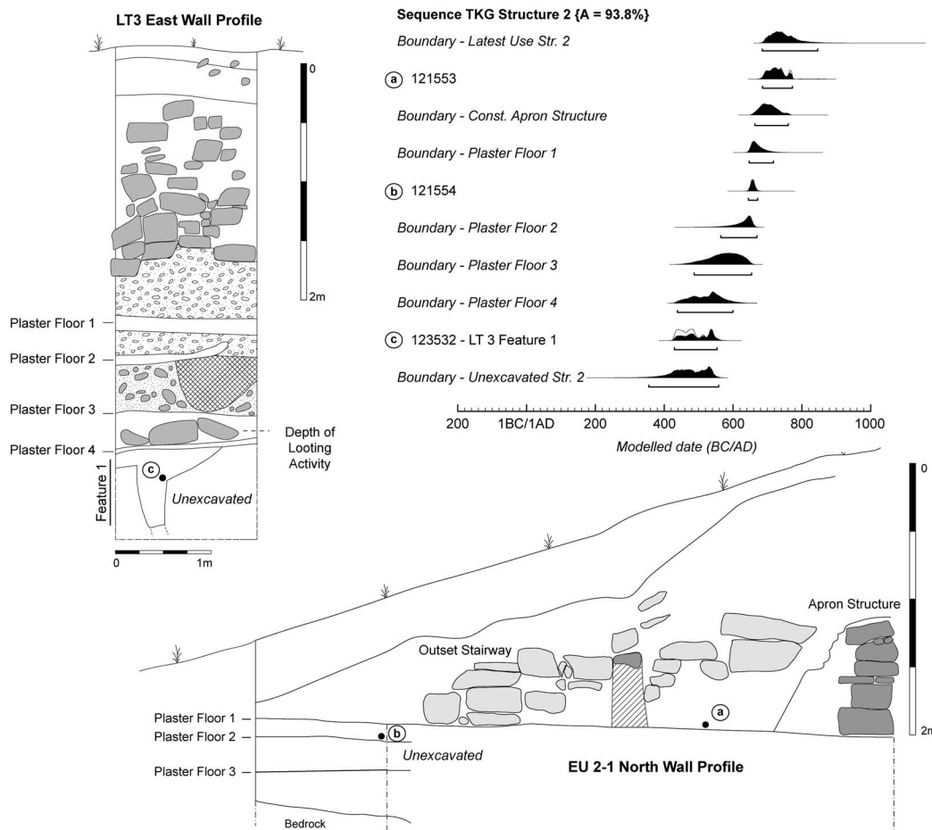
Figure 7 Profiles of EU 2-1 and LT3 at Tzutziiy K'in Structure 2, showing locations of 14 C samples and modeled calibrations.
