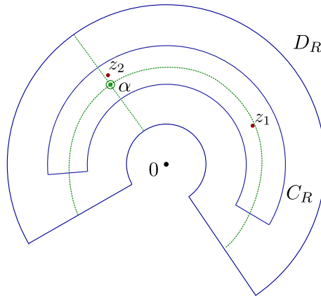
FIGURE 1. Illustration of the proof of Lemma 2.12, showing the point \alpha , the boundary of the disk \Delta(\alpha, R/20) and the four arcs I_i .
