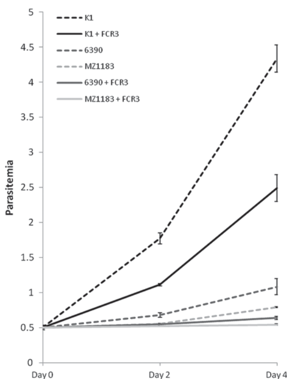
Fig. 2. Native Peruvian strains in competitive assays; comparative growth of clones when alone versus co-cultured with FCR3. FAM fluorescence shows the growth of K1 genotype clones K1, 6390 and MZ1183. Solid line shades illustrate clones in a 50/50 co-culture with FCR3 whereas dotted lines represent single-clone controls.
