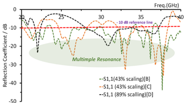
Figure 4. Array antennae A, B, C, and D with some fractal fragments through scaling down with 43%,43%, and 89%, in range of 20–40 GHz.
