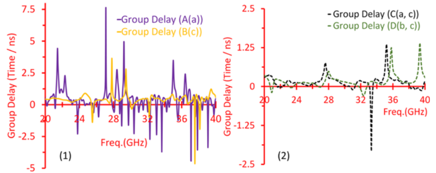
Figure 10. Group delay vs frequency graph for proposed antennae concerning A, B, C, and D.
