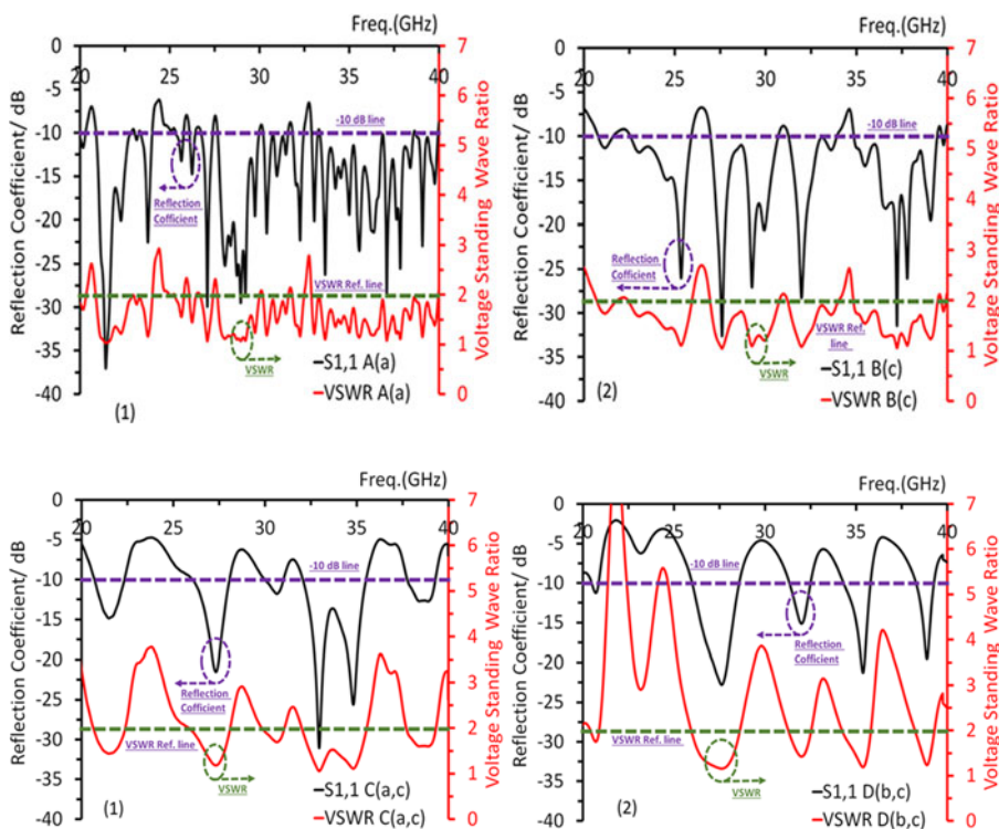
Figure 6. S_{11} , VSWR, vs frequency graph for proposed antennae A and B, respectively. VSWR = voltage standing wave ratio.
