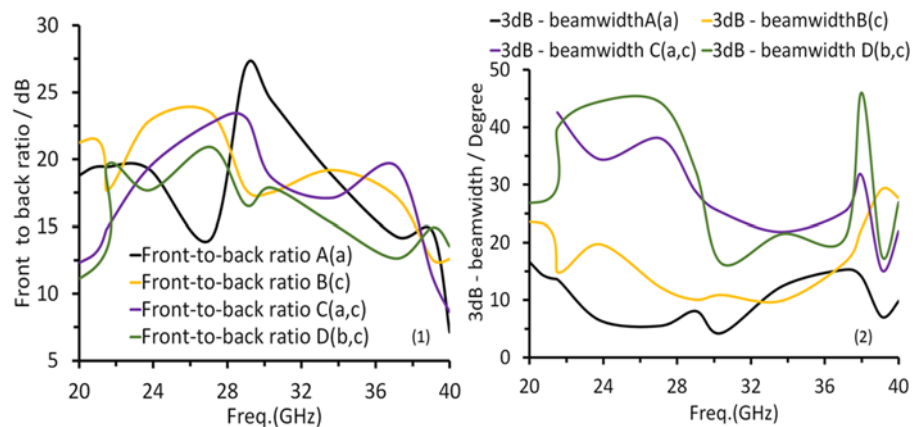
Figure 8. FBR, 3 dB beam-width vs frequency graph for proposed antennae with A, B, C, and D. FBR = front-to-back ratio.
