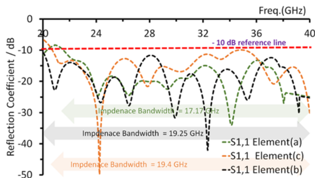
Figure 2. Element antennae a, b, and c with some fractal fragments in the range of 20–40 GHz.
