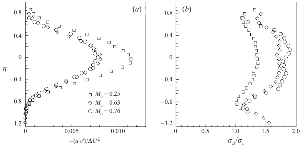
FIGURE 16. (a) Mean profiles of Reynolds stress and (b) perturbation asymmetry.
