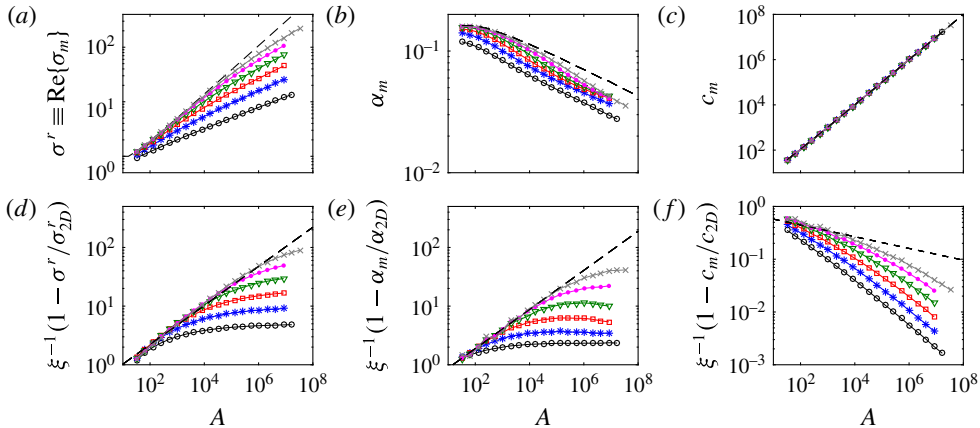
FIGURE 6. (Colour online) Data (dots) as a function of A , for different aspect ratios \xi . (a–c) The maximum growth rate \sigma^r \equiv \text{Re}\{\sigma_m\} , with the corresponding vertical wavenumber \alpha_m and the propagation speed c_m , together with the two-dimensional results (black dashed lines), which exhibit asymptotic scalings of \text{Re}\{\sigma_{2D}\} \sim A^{4/9} , \alpha_{2D} \sim A^{-1/9} and c_{2D} \sim A as A \rightarrow \infty . (d–f) The relative deviation from the two-dimensional results, scaled by the aspect ratio \xi , for the same three quantities. The dashed lines show the asymptotic predictions for \xi \rightarrow 0 taken from (4.13) (see asymptotic analysis in § 4). The quantities deviate from the asymptotic predictions as A \rightarrow \infty , as discussed in § 4.3. The different symbols correspond to \xi = 1/5 (black circles), \xi = 1/10 (blue stars), \xi = 1/20 (red squares), \xi = 1/40 (green triangles), \xi = 1/80 (pink dots) and \xi = 1/160 (grey crosses).
