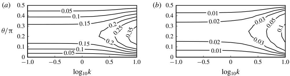
FIGURE 5. The contours of J_{min} in the wavenumber plane approximated with two methods: (a) J_{min} is approximated by the minimum of J for all DU_0 = \sum_{0 \leq m \leq 5} a_m T_m(y) , where T_m is the Chebyshev polynomial of degree m , and |a_m| \leq 5 ( 0 \leq m \leq 5 ) are integers; (b) J_{min} is approximated by the local minimum of J among all DU_0 = \sum_{0 \leq m \leq 15} a_m T_m(y) with a gradient descent method.
