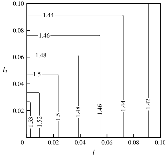
FIGURE 2. The contours of k_0 in the (l, l_T) plane.
