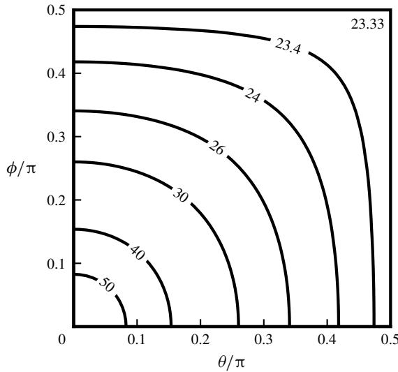
FIGURE 6. The contours of R'_1 for DU_0 = D\tilde{T}_0 = 1 , k = 1 , \lambda = 1 and l = l_T = 0 . The boundaries \theta = \pi/2 and \phi = \pi/2 constitute the contour R'_1 \approx 23.33 .
