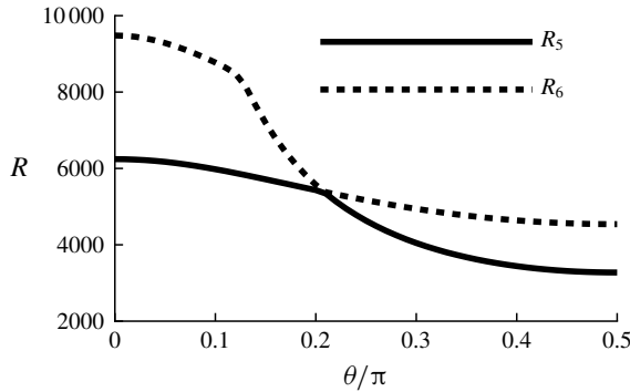
FIGURE 1. The fifth and sixth positive eigenvalues for the energy stability of the parallel shear flow with DU_0 = \sin(8\pi y) , Pr D\tilde{T}_0 = 0 , l = 0 and k = 1 .
