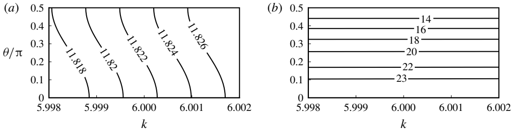
FIGURE 4. The contours of R_1 (a) and (1 + \cos \theta)R_1 (b) for the energy stability of the mixed convection with DU_0 = \cos(\pi y) + \cos(3\pi y) , Pr D\tilde{T}_0 = 10 \sin(\pi y) , \lambda = 1 and l = l_T = 0 .
