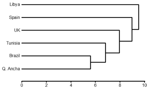
Figure 9. Dendrogram (cluster analysis) comparing Upper Silurian miospore assemblages of Brazil (Stemans, Rubinstein & Melo, 2008), Libya (Rubinstein & Stemans, 2002), Spain (Richardson, Rodríguez & Sutherland, 2001), Tunisia (Spina & Vecoli, 2009), the UK (Richardson & Lister, 1969; Richardson & McGregor, 1986; Burgess & Richardson, 1995) and Quebrada Ancha (present study). x -axis represents the Euclidean distance.
