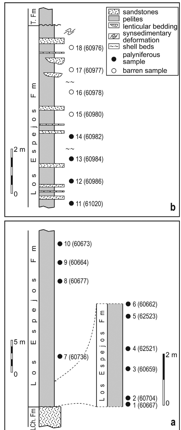
Figure 2. Stratigraphic sections of the studied of Los Espejos Formation in the Quebrada Ancha area. (a) Lower section. (b) Uppermost section. Location and identification numbers of palynological samples in both sections, and the position of the third faunal assemblage of Benedetto et al. (1992) – mainly represented by Coelospira extensa – are indicated.
