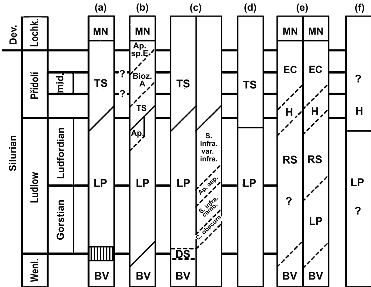
Figure 3. Miospore biostratigraphic zonal correlations in the Upper Silurian and the Lochkovian. (a) Richardson & McGregor (1986); (b) Richardson & Edwards (1989); (c) Burgess & Richardson (1995); (d) Rubinstein & Steemans (2002); (e) Richardson, Rodríguez & Sutherland (2001); (f) Hassan Kermadji (2007). Diagonal lines indicate boundaries revised herein. The exact position of biozones and sub-biozones with their correlation with series and stage boundaries remain doubtful because of the lack of reliable independent biostratigraphic control. BV – brevicosta-verrucatus ; DS – downiei-sagittarius ; LP – libycus-poecilomorphus ; RS – reticulata-sanpetrensis ; H – hemisferica ; TS – tripapillatus-spicula ; EC – elegans-cantabrica ; MN – micronatus-newportensis .
