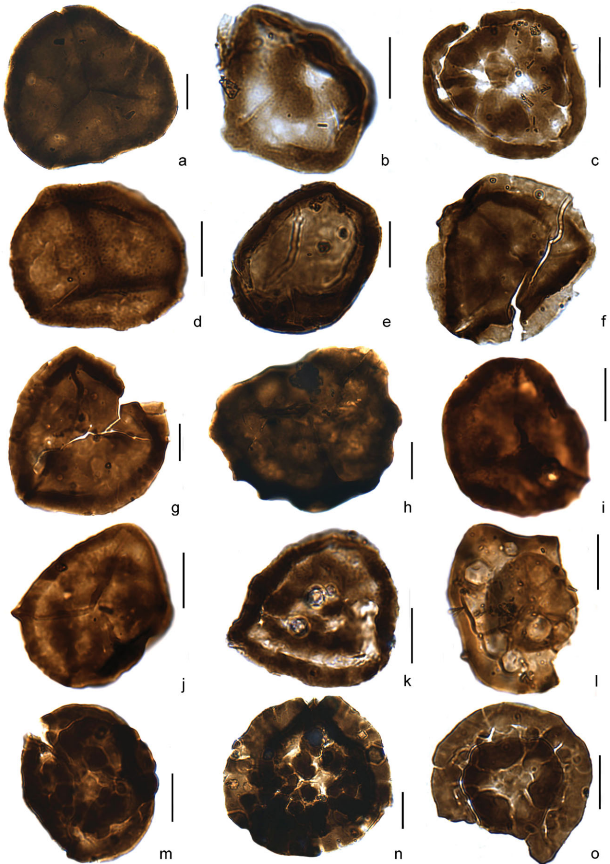
Figure 6. (Colour online) (a) Ambitisporites avitus/dilutus sensu Steemans, Le Hérissé & Bozdogan, 1996, slide 60659, K45/3. (b) Amicosporites? sp., slide 60986, M45/0. (c) Amicosporites streelii Steemans, 1989, slide 60984, S29/1. (d) Apiculiretusispora sp., slide 60664, F41/2. (e) Archaeozonotriletes chulus (Cramer) Richardson & Lister, 1969, slide 60986, L29/4. (f, g) Breconisporites sp. B in
