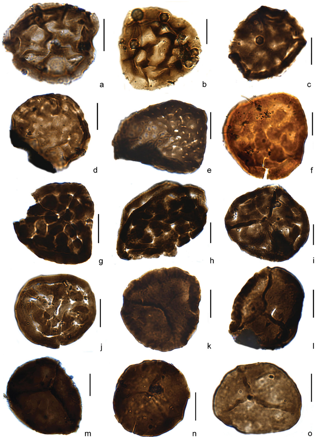
Figure 7. (Colour online) (a, b) Chelinospora cf. C. hemisferica in Richardson, Rodríguez & Sutherland, 2001; (a) slide 60677, K33/3; (b) 62521, S31/2. (c) Chelinospora cf. C. cantabrica Richardson, Rodríguez & Sutherland, 2001, slide 62521, O30/3. (d) Chelinospora obscura Burgess & Richardson, 1995, slide 60659, J25/2. (e) Chelinospora sanpetrensis (Rodríguez) Richardson, Rodríguez & Sutherland, 2001, slide 60664, W45/2. (f–j) Chelinospora verrucata var. verrucata morphon; (f) slide 60984, H39/2; (g) slide 60704,
